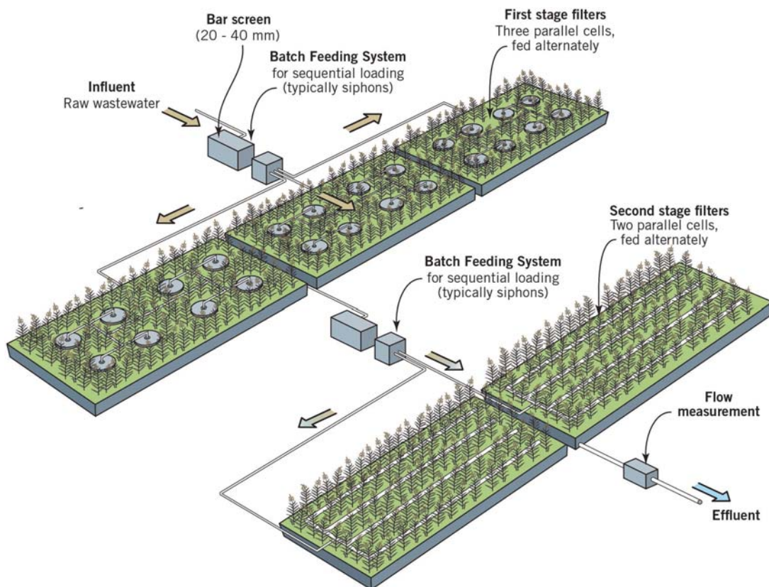
Figure 5.4 Schematic of the classical French VF design (Dostro et al. , 2017).
