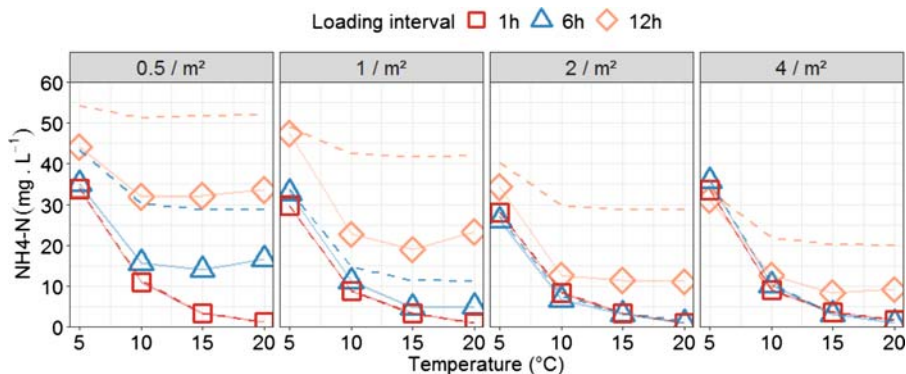
Figure 5.2 Simulated \text{NH}_4\text{-N} effluent concentrations of a VF filter with main layer of coarse sand (1–4 mm) for at an OLR of 80 \text{ g COD/m}^2/\text{d} for different loading intervals and different number of holes in the distribution pipes (median concentrations: symbols; maximum concentrations: dashed lines).
