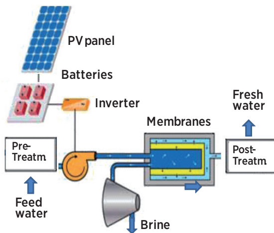
Figure 4 – Coupled PV and RO desalination plants (Al-Karaghoul et al., 2011)
