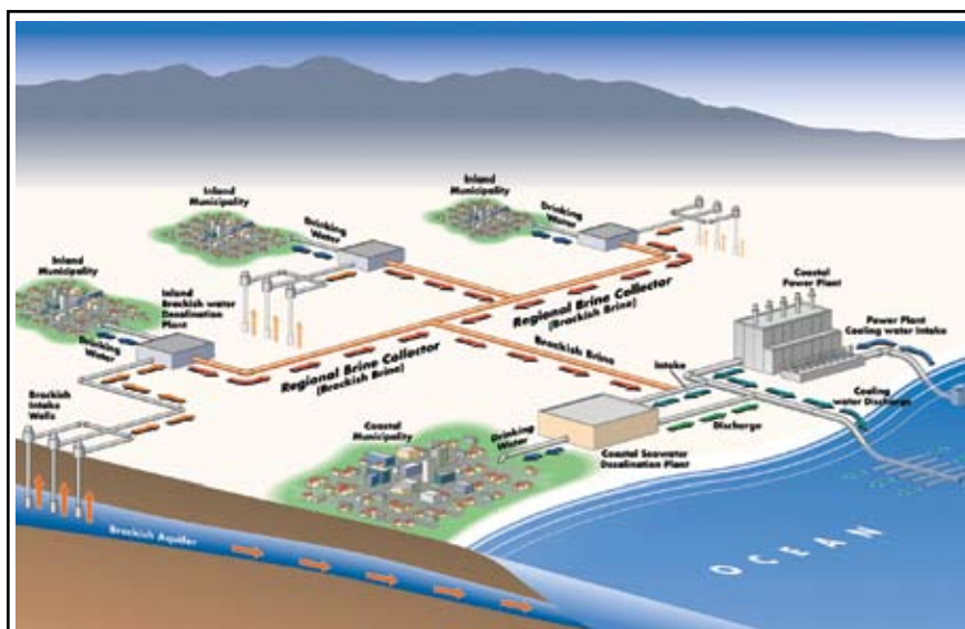
Figure 1. Integrated inland desalter brine disposal and seawater desalination.
