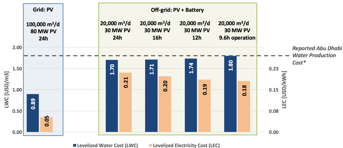
* As reported by the Abu Dhabi Regulation and Supervision Bureau and adjusted to exclude transmissions and distribution cost. Figure 5.4: Estimated cost of water for multiple solar powered seawater desalination scenarios in the UAE 164 .
