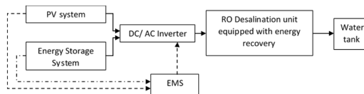
Figure 3.1: Standalone operation
