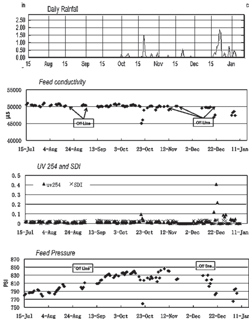
Figure 10.2. Environmental, water quality, and operational parameters collected at Carlsbad desalination pilot plant.
