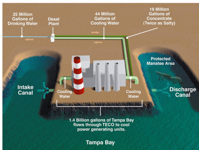
Fig. 9. Collocation configuration of Tampa Bay Seawater Desalination Plant.
