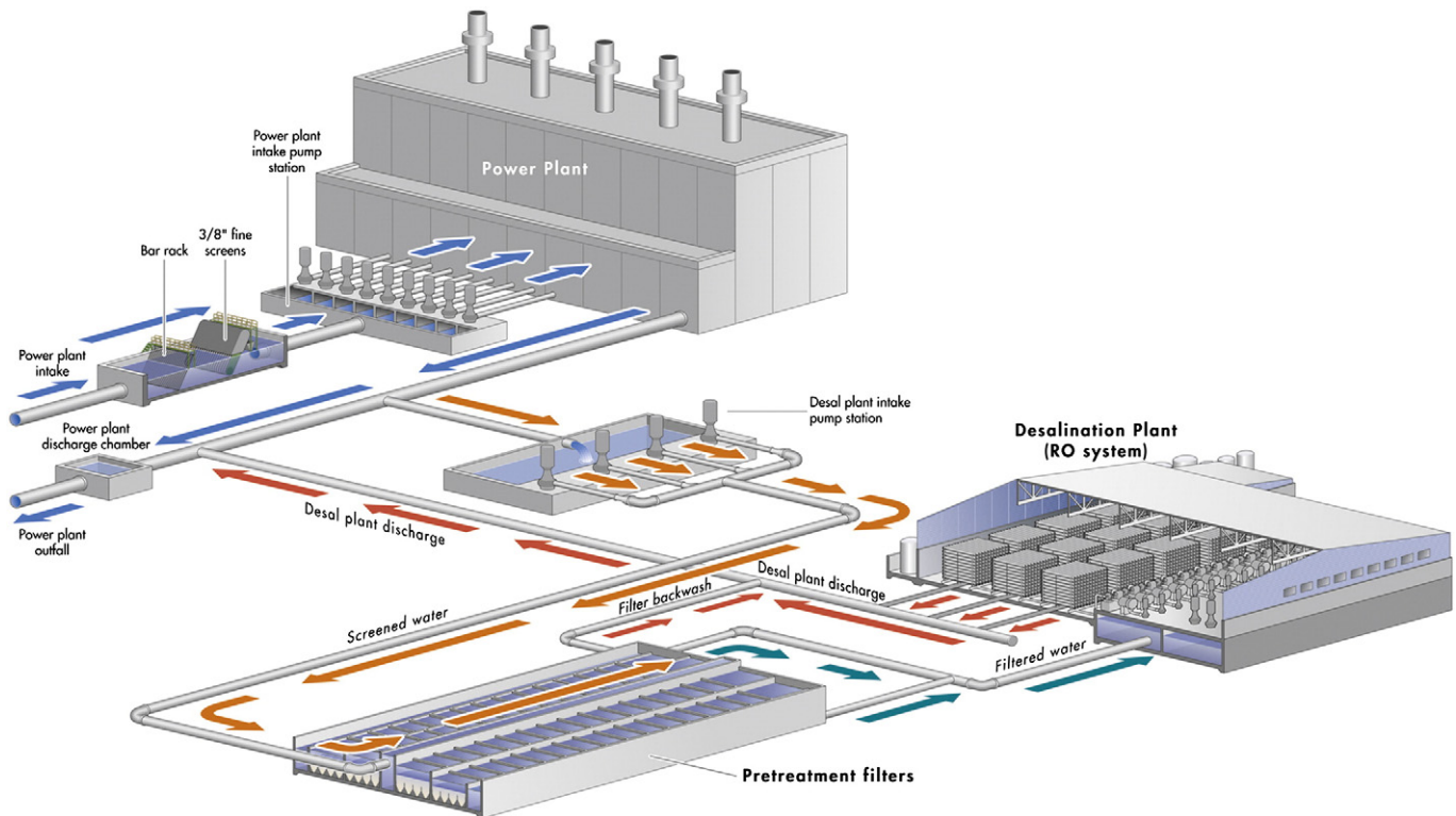
Fig. 7. Collocation of SWRO Plant and Coastal Power Generation Station.
