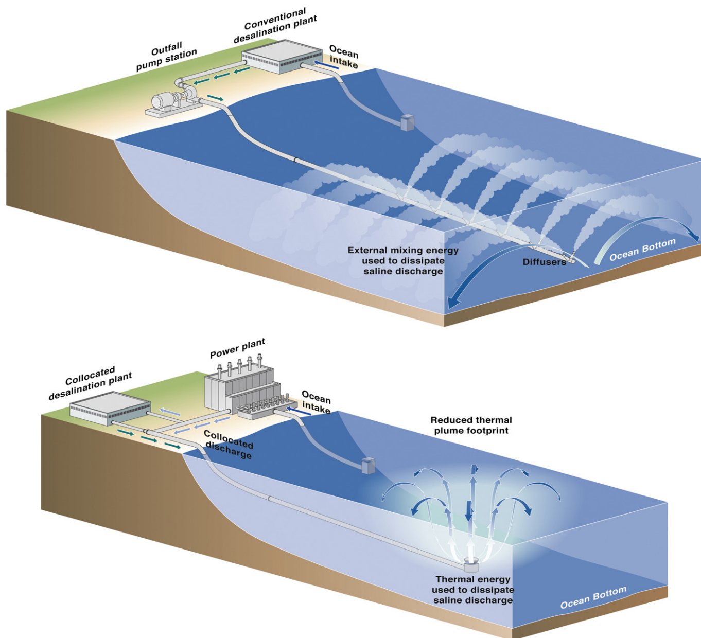
Fig. 8. Comparison of conventional and collocated concentrate discharges.
