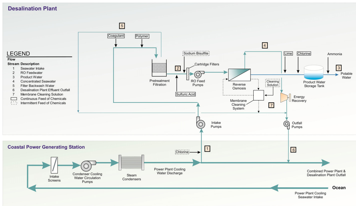
Fig. 1. Schematic of Carlsbad seawater desalination plant.
