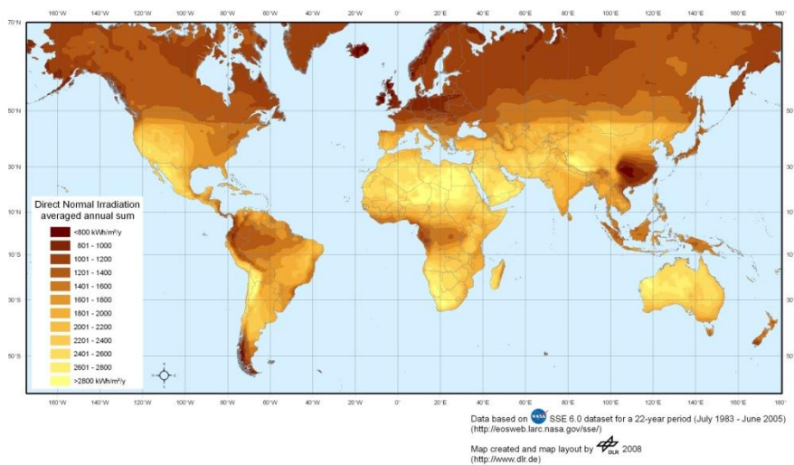
Direct Normal Irradiation (DNI)
