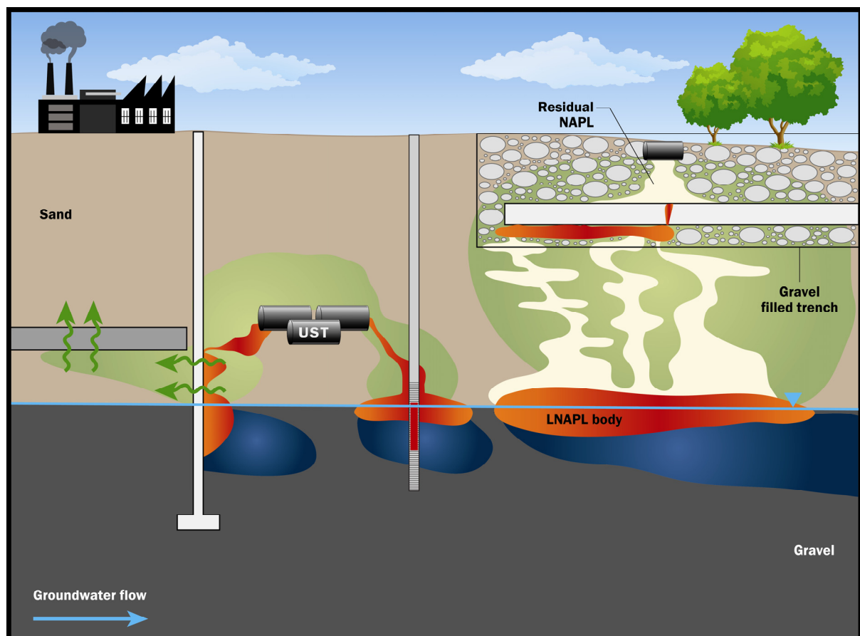
Figure 5.11. LNAPL release into made ground.
