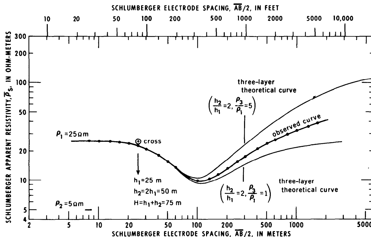
Figure 35.—Interpretation of a three-layer Schlumberger H-type curve.
