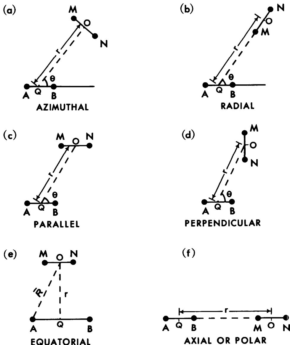
Figure 6.—Dipole-dipole arrays. The equatorial is a bipole-dipole array because AB is large.
