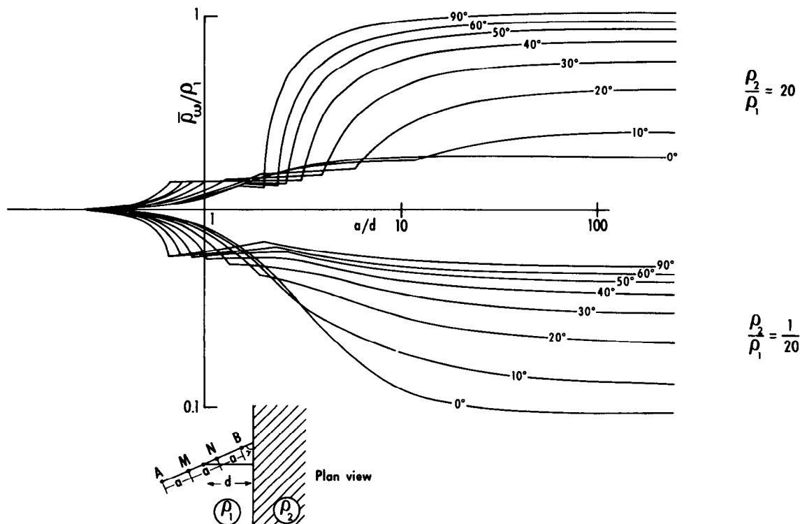
Figure 21.—Examples of the variation of Wenner sounding curves across a vertical contact at various azimuths. Unpublished data calculated by Zohdy, 1970. a , Wenner spacing; d , perpendicular distance from center of array to surface trace of vertical contact; \bar{\rho} , apparent resistivity; \rho , true resistivity.
