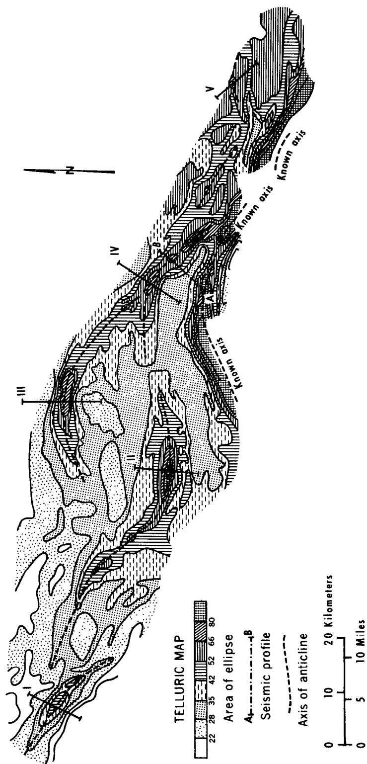
Figure 3.—Telluric map of the Aquitaine basin, France.
