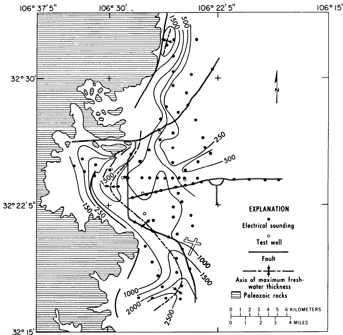
Figure 47.—Map of White Sands area, New Mexico, showing isobaths of the lower surface of fresh-water aquifer. Datum is land surface (after Zohdy and others, 1969).
