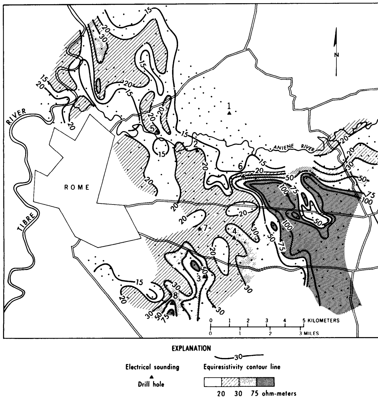
Figure 23.—Map of apparent resistivity near Rome, Italy (after Breusse, 1961a).
