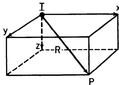
Figure 4.—Diagram showing the relationship between a point source of current I (at origin of coordinates) in an isotropic medium of resistivity \rho and the
