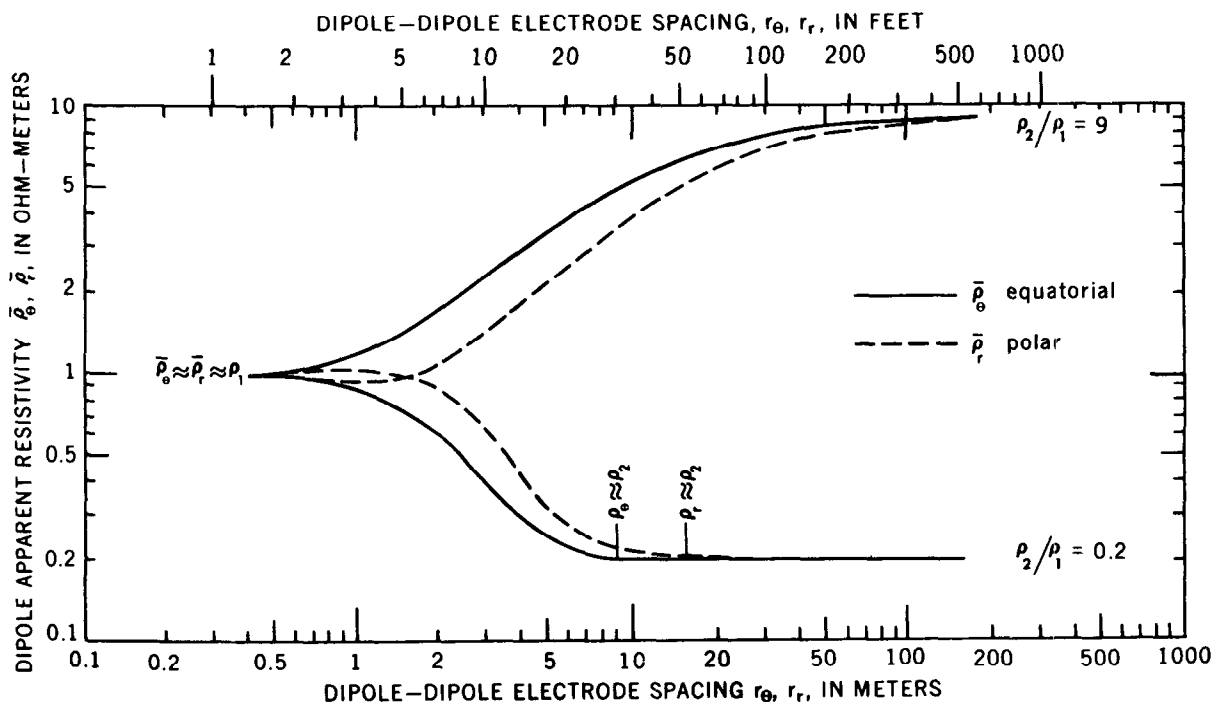
Figure 17.—Comparison between two-layer azimuthal (or equatorial) and radial (or polar) sounding curves ( h_1 = 1 meter (3.28 feet), \rho_2/\rho_1 = 9 or 0.2).
