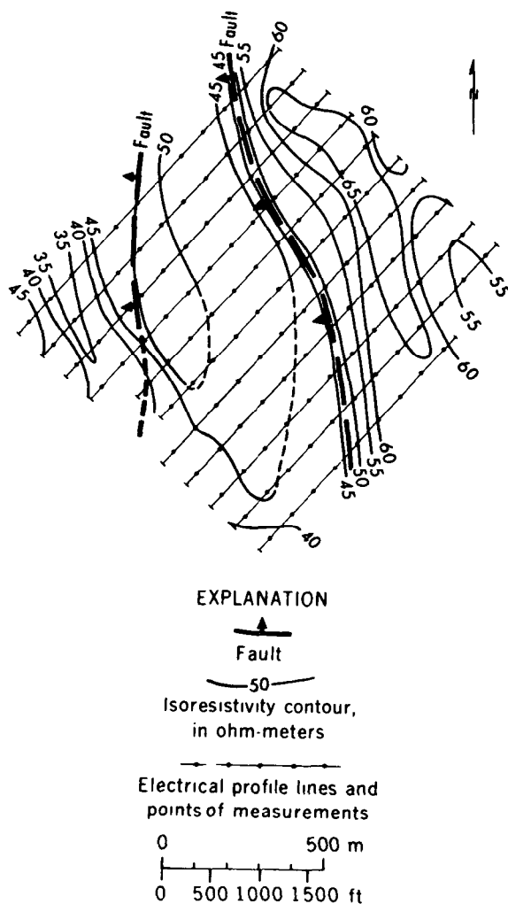
Figure 44.—Map of apparent resistivity in the Bad-Krozingen geothermal area, Germany. AB = 4,000 m (13,120 feet) (after Breusse and Astier, 1961).
