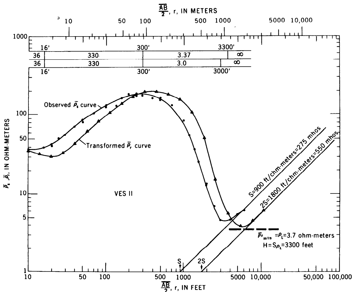
Figure 28.—Transformation of a Schlumberger KH-type curve into a polar dipole-dipole curve to evaluate \bar{\rho}_{rms} = \rho_i and H = S\rho_i (after Zohdy, 1969a). Reproduced with permission of "Geophysics."
