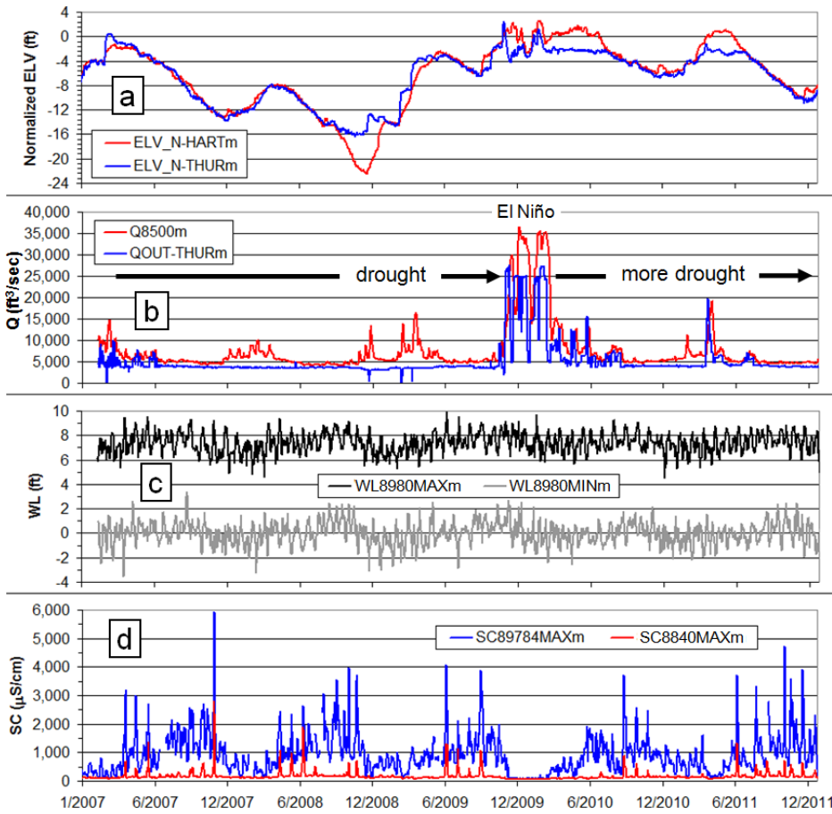
Figure 2. Hydrographs showing the measured data used in the study: a) normalized water elevations (ELV) for Lakes Hartwell and Thurmond (ELV_N-HARTm, ELV_N-THURm), b) flow (Q) from Lake Thurmond outflow (QOUT-THURm) and streamflow at USGS gage 02198500 (Q8500m), c) maximum and minimum water levels (WL) at USGS gage 02198980 (WL8980MAXm, WL8980MINm), and d) maximum specific conductance (SC) at USGS gages 021989784 (SC89784MAXm) and 02198840 (SC8840MAXm).
