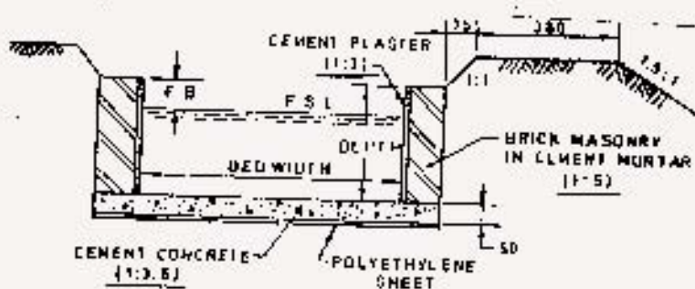
FIG. 3. TYPICAL CEMENT CONCRETE AND BRICK MASONRY SECTION
