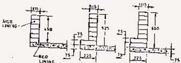
FIG. 2 TYPICAL SECTIONS OF SHIELD WALLS
