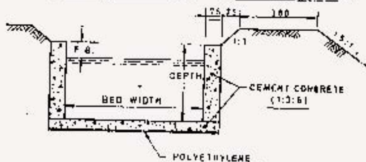
FIG. 4. TYPICAL CEMENT CONCRETE SECTION
