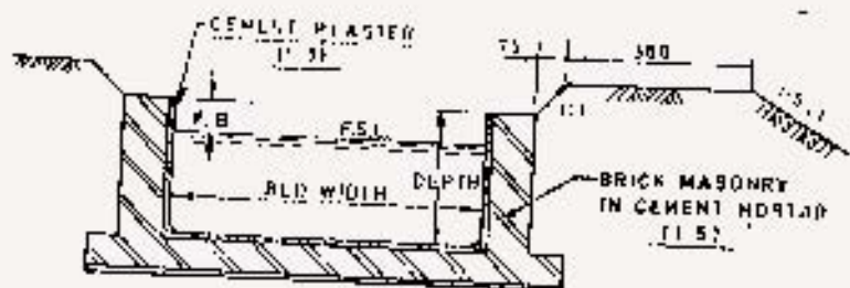
FIG. 1. TYPICAL BRICK MASONRY SECTION
