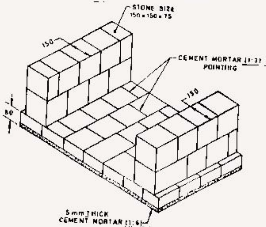
FIG. 5 STURGE MASONRY BRIDGE
