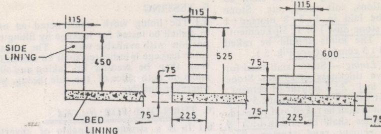
All dimensions in millimetres. FIG. 2 TYPICAL SECTION OF SIDE WALLS
