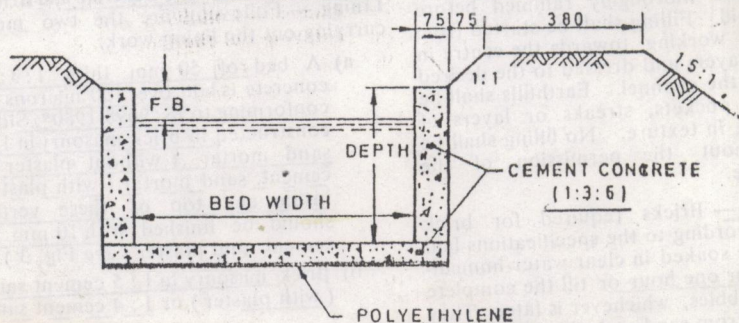
All dimensions in millimetres. FIG. 4 TYPICAL CEMENT CONCRETE SECTION
