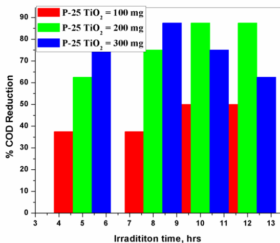
Figure.4. Optimization of catalyst concentration using P-25 \text{TiO}_2 for the degradation of GOV
