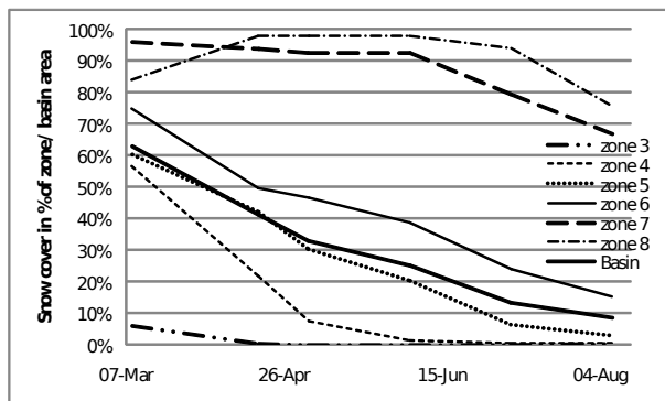
Fig. 2 Snow depletion curves for Indus sub basin
