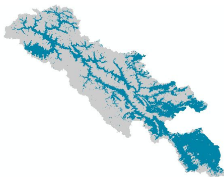
Fig. 3 Snow extent in March 2007
