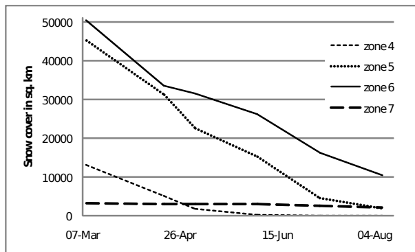
Fig. 1 Snow extent depletion in elevation zones
