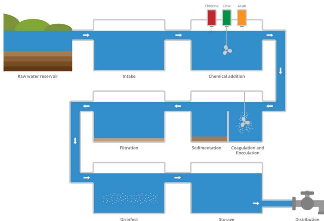
Figure 2: Drinking water treatment process.
