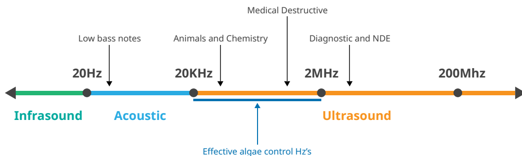
Figure 4: Sound frequencies.
