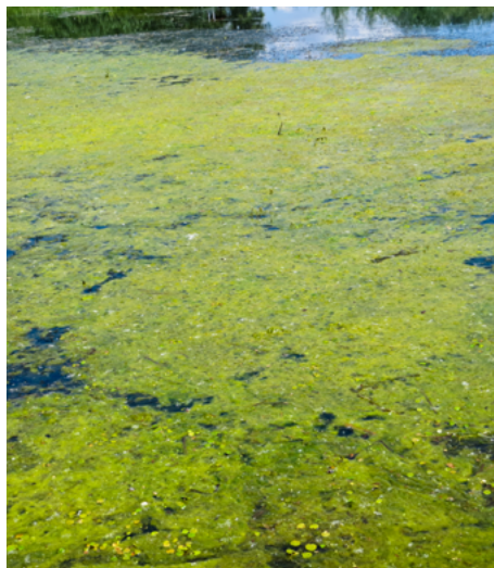
Figure 10: Filamentous algae.
