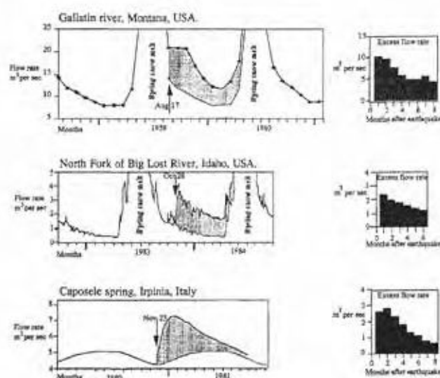
Figure 2 Fluvial hydrological signatures for three major normal fault earthquakes showing seismohydraulically induced rise in water-tables
