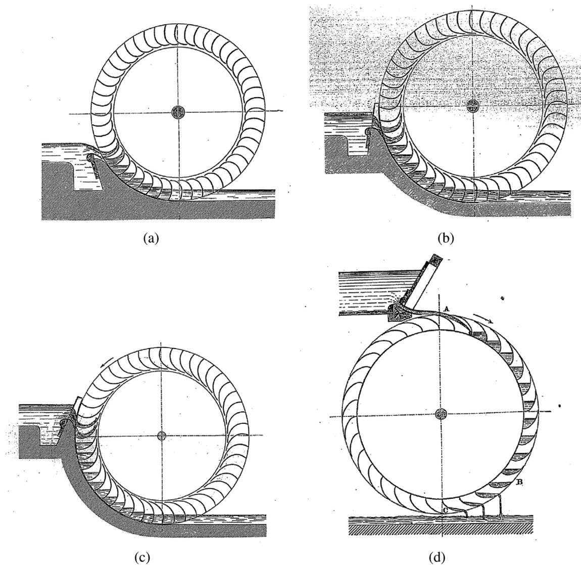
Fig. 2. Historic representations of gravity water wheels [49]: (a) low breastshot/undershot, (b) middle breastshot, (c) high breastshot and (d) overshot.
