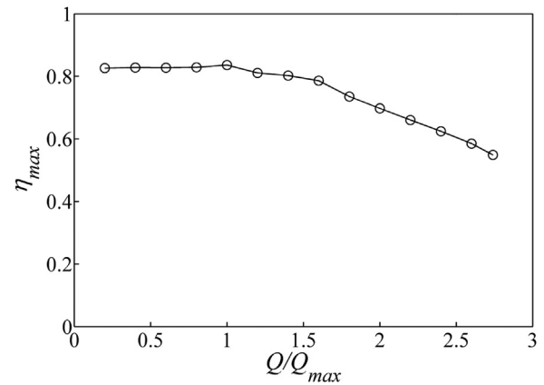
Fig. 8. Efficiency of overshoot water wheels as a function of the normalized flow rate, where Q_{max} is the flow rate at maximum efficiency [52].
