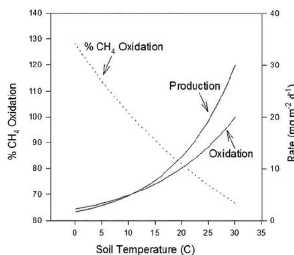
Figure 3.4.4 A model illustrating the potential for \text{CH}_4 oxidation to decline as a fraction of methane production with increasing temperature (Magonigal, 1996).
