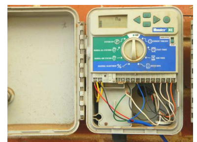
Feed the red, black, blue and green wires into the controller
