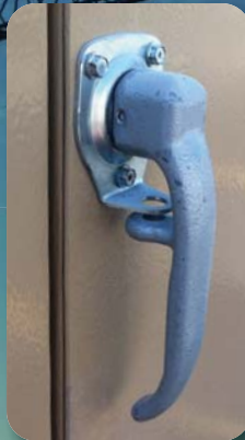
3 Point door latch with "L" handle and pad lockable
