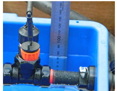
Measuring the depth of water in the evaporator at the low level for UMIC
