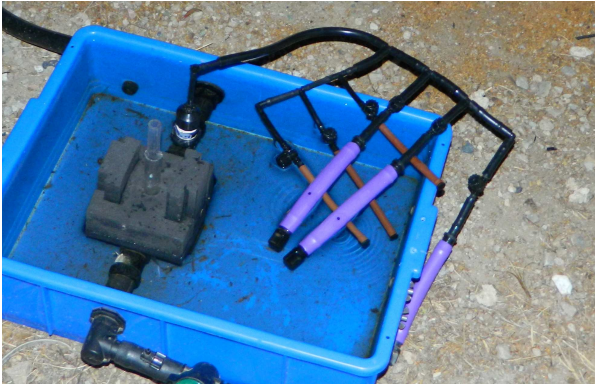
Precision adjustable dripper with 3 Netafim Miniscape drippers and 3 Netafim Bioline drippers.
