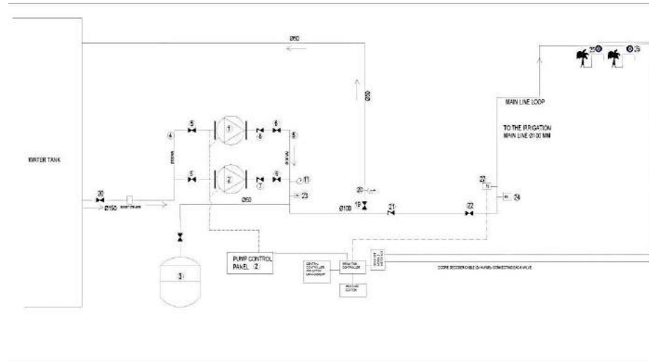
IRRIGATION SYSTEM LINE DIAGRAM
