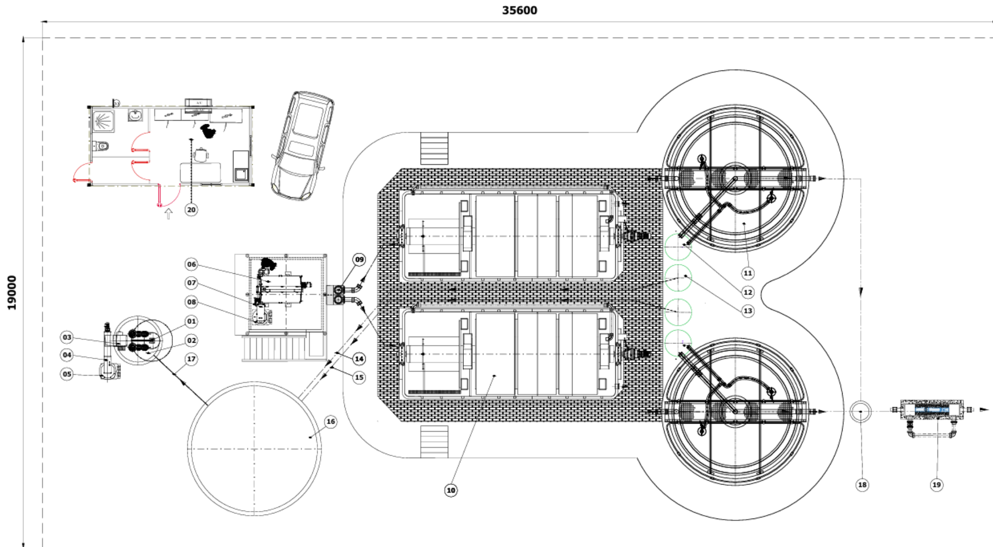
View from above, WWTP 1500 PE with Ø3m BioDisk unit for ABOVE-GROUND installation and removable if necessary to another site. The final settlement tank is sealed in concrete.
