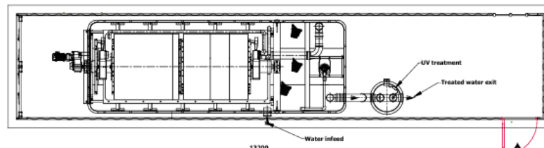
100 SHR unit installed in a 40 Ft container
