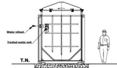
SHR 100 unit, seen from behind
