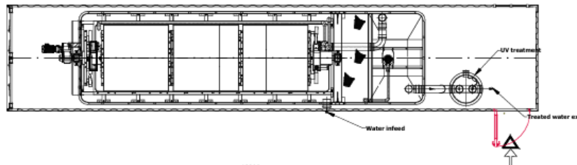
150 SHR unit installed in a 40 Ft container
