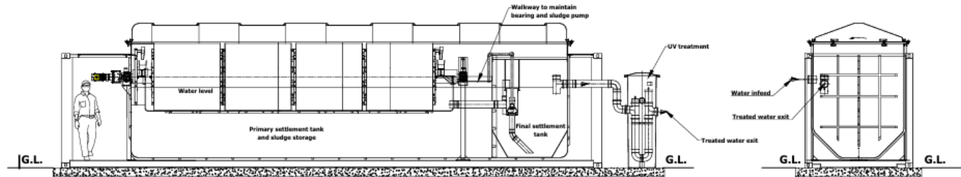
200 SHR unit installed in a 40 Ft container
