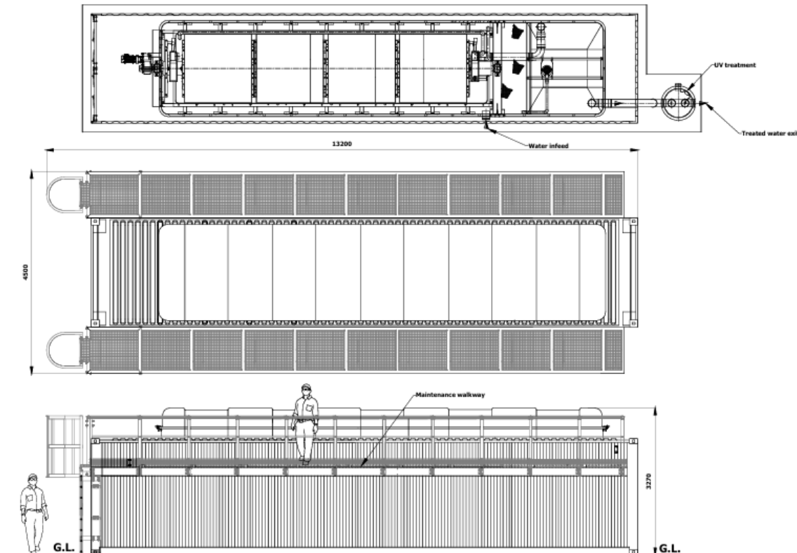
200 SHR unit installed in a 40 Ft container
