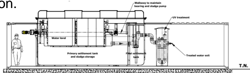
100 SHR unit installed in a 40 Ft container
