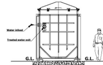
SHR 150 unit, seen from behind
