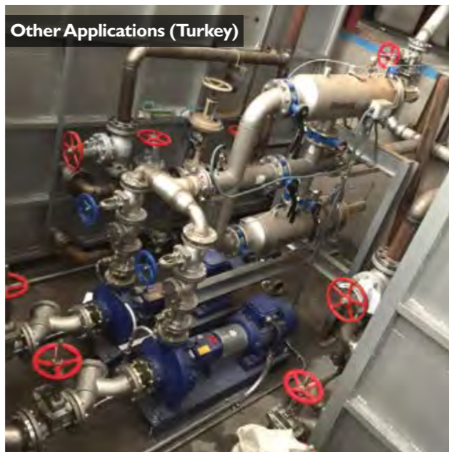
Plastic Industry, Process Water Filtration (Turkey)
