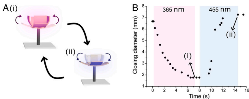
Fig. 3. Light-driven artificial polyp. (A) Light-driven reversible deformation of polyp-like design with the gripper composed of two orthogonally placed LCNs (10 mol % azobenzene) upon exposure to (i) UV and (ii) blue light. (B) Analysis of the closing diameter of the gripper upon exposure to UV light (75 mW/cm 2 ). Ceasing UV light exposure results in a stable closed state. Reopening is triggered by blue light.
