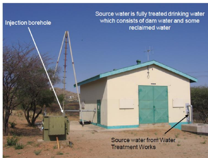
Figure 29 - Injection borehole site with indication of source water (Murray, 2017).
