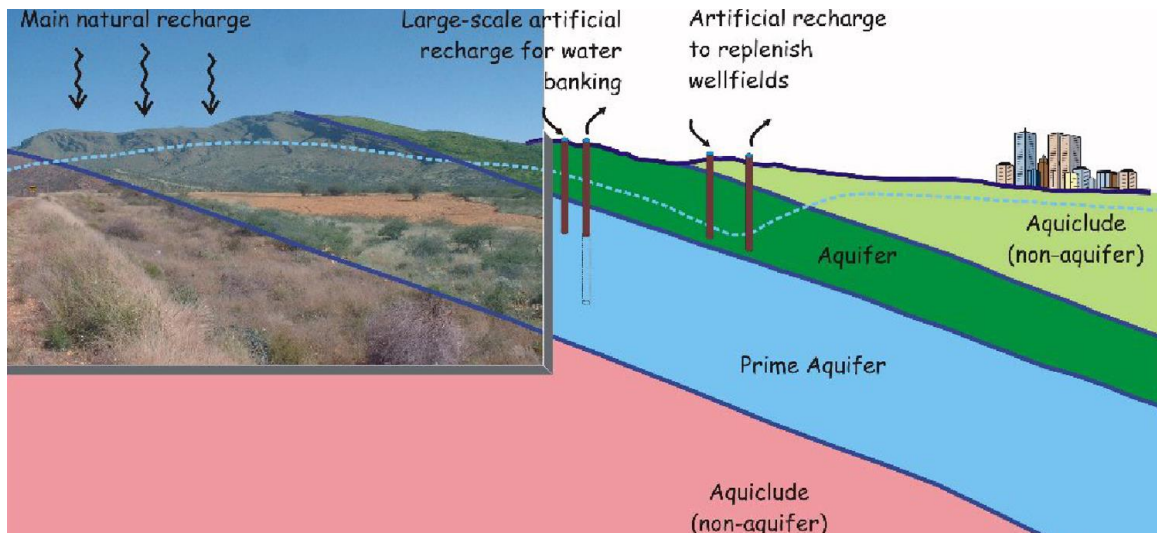
Figure 33 - Schematic of the main lithologies and injection areas (Murray, 2017).
