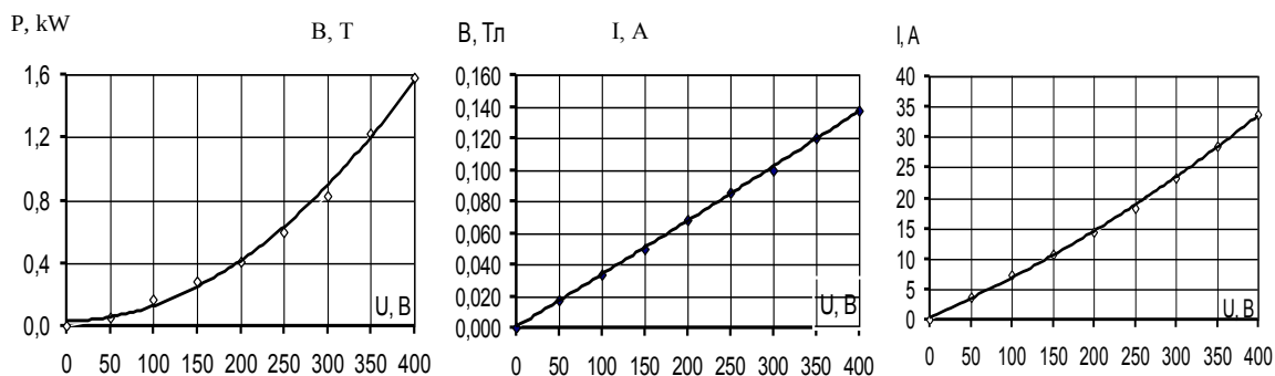
Fig. 6. Dependency of main characteristics of a salient pole rotating electromagnetic field inductor on voltage in windings (bore diameter – 100 mm, core length – 100 mm)
