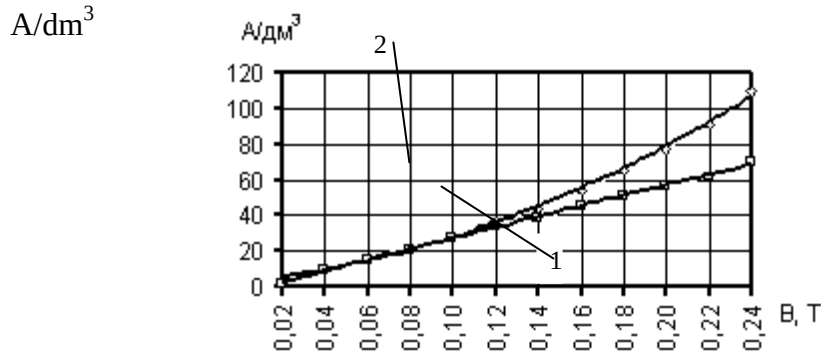
Figure 5. The current consumed by inductor windings to obtain required induction in the center of the inductor bore
