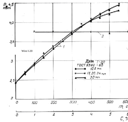
Fig. 12. Influence of weight and dimensions of FE on power consumption in AVS (inductor bore diameter 100 mm, ferromagnetic elements made of spring wire d = 2 mm):
