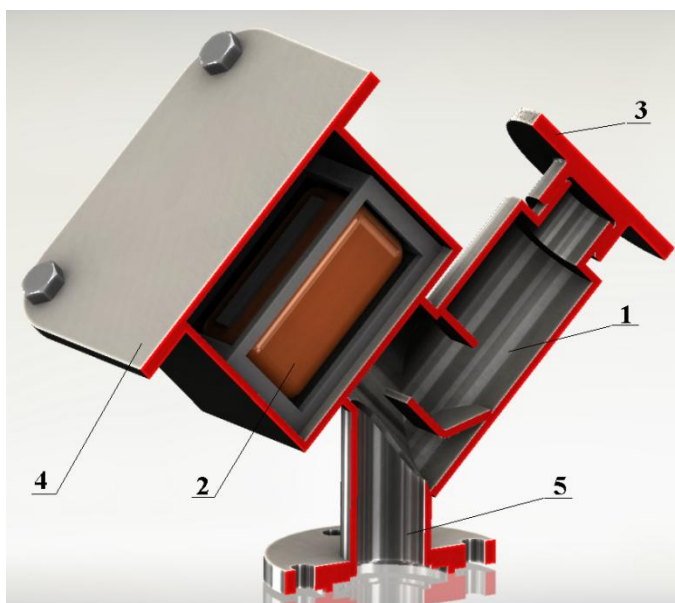
Fig. 11. Ferromagnetic element portioner:
