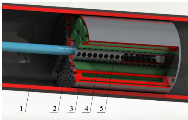
Fig. 9. AVS chamber with tubes: 1 – chamber; 2 – mesh; 3 – bush; 4 – tubes; 5 – filter tube.
