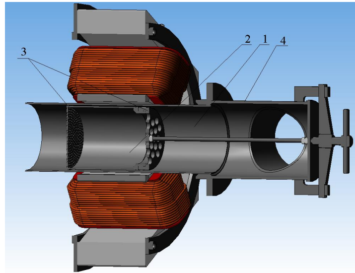
Fig. 7. The chamber of AVS for liquid phase processes: 1 – chamber; 2 – bush; 3– strainer;
