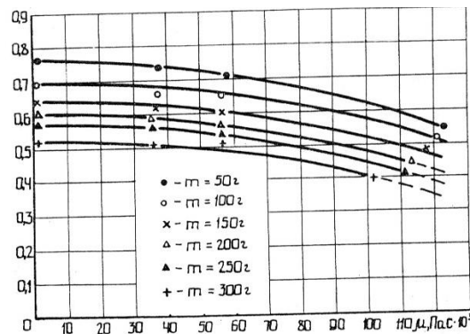
Fig. 17. Dependence of critical flow velocity on kinetic product viscosity coefficient ( D_{\text{external}} = 76 \text{ mm} ; H = 11,8 \cdot 10^4 \text{ A/m} ; ferromagnetic elements: steel 08G2S, d = 2 \text{ mm} , \ell/d = 10 )
