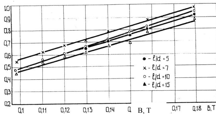
Fig. 19. Dependency of the critical flow velocity on the magnetic induction with various l/d ratios
