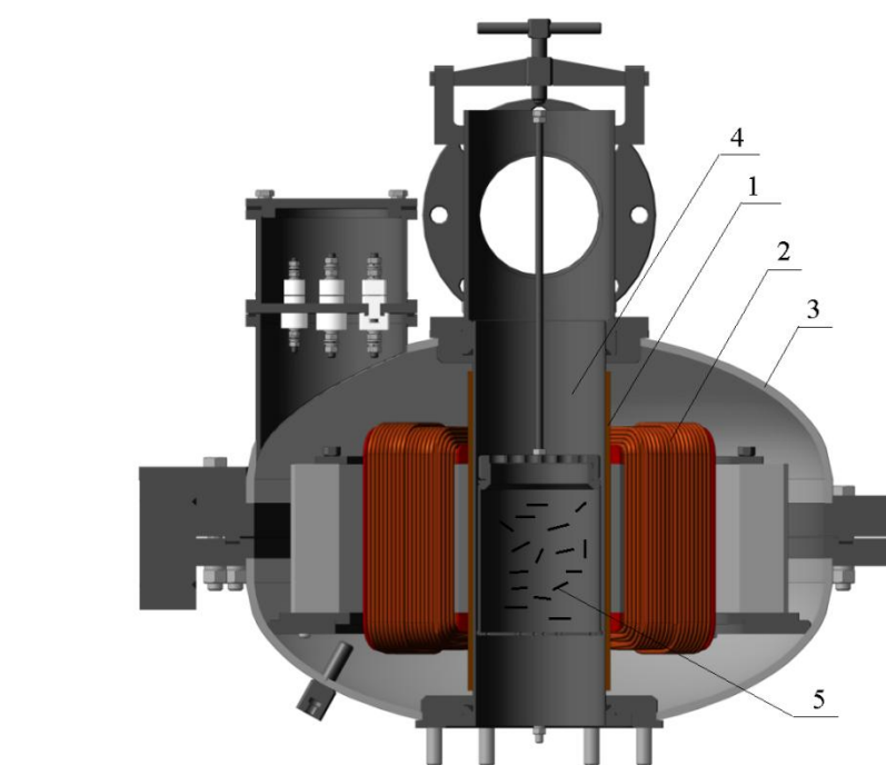
Fig. 3. Electromagnetic vortex system: 1 – protective bushing; 2 – inductor of rotating electromagnetic field; 3 – inductor body; 4 – non-magnetic material work operating chamber; 5 – ferromagnetic elements
