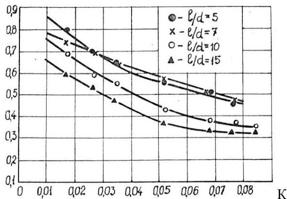
Fig.14. Dependency of critical flow velocity on chamber filling coefficient ( D_{ch} = 76 \text{ mm} ; H = 11,8 \cdot 10^4 \text{ A/m} ), ferromagnetic elements:
