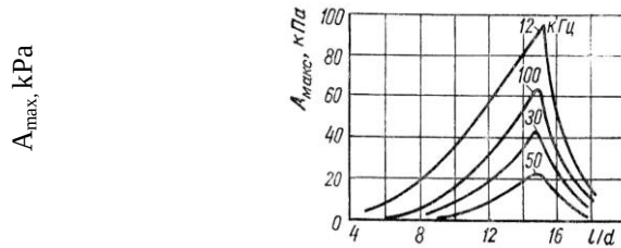
Fig. 22. Dependency of the maximum amplitude of acoustic wave pressure on the \ell / d ratio for nickel ferromagnetic elements d = 1 mm
