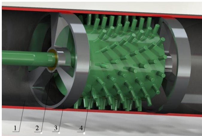
Fig. 10. AVS chamber with rotor:
