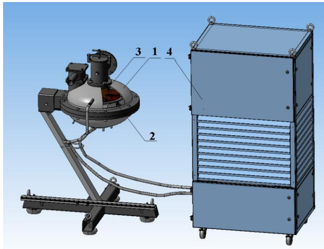
Fig. 2 AVS -150. Internal inductor diameter 150 mm, operating chamber diameter 136 mm. 1 – inductor body; 2 – EMF inductor; 3 – operating chamber; 4-controls.
