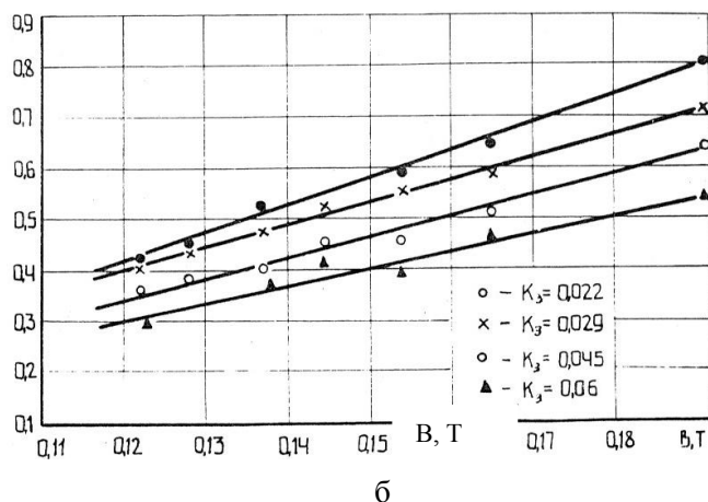
Fig. 18. Dependency of the critical flow velocity on the magnetic induction with varying chamber filling coefficients:
