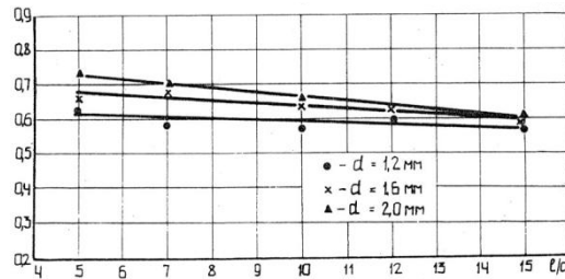
Fig. 16. Dependency of critical flow velocity on \ell/d ratio for various diameters of ferromagnetic elements ( D_{\text{external}} = 76 \text{ mm} ; H = 11,8 \cdot 10^4 \text{ A/m} ); ferromagnetic elements: steel 08G2S, m = 150 \text{ g} )
