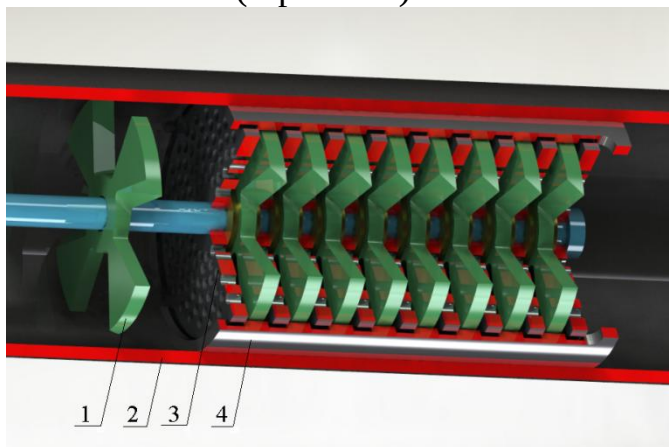
Fig. 8. AVS chamber with knives: 1 – knives; 2 – chamber; 3– mesh filter; 4 – bush.
