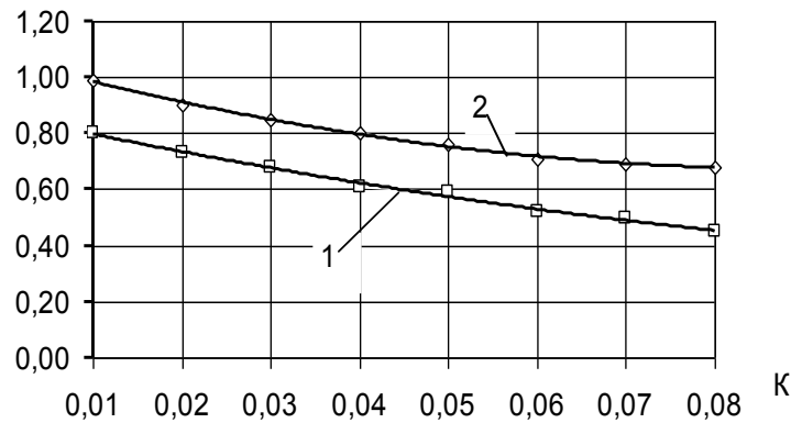
Fig. 20. Dependency of critical flow velocity on chamber filling coefficient (D_{int} = 121 \text{ mm}; H = 12,3 \cdot 10^4 \text{ A/m}; \text{ferromagnetic elements: steel 08GS, } d = 2 \text{ mm, } l/d = 10: 1 – horizontal chamber alignment; 2 – vertical chamber alignment
