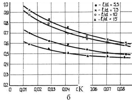
Fig.14. Dependency of critical flow velocity on chamber filling coefficient ( D_{ch} = 76 \text{ mm} ; H = 11,8 \cdot 10^4 \text{ A/m} ), ferromagnetic elements:
