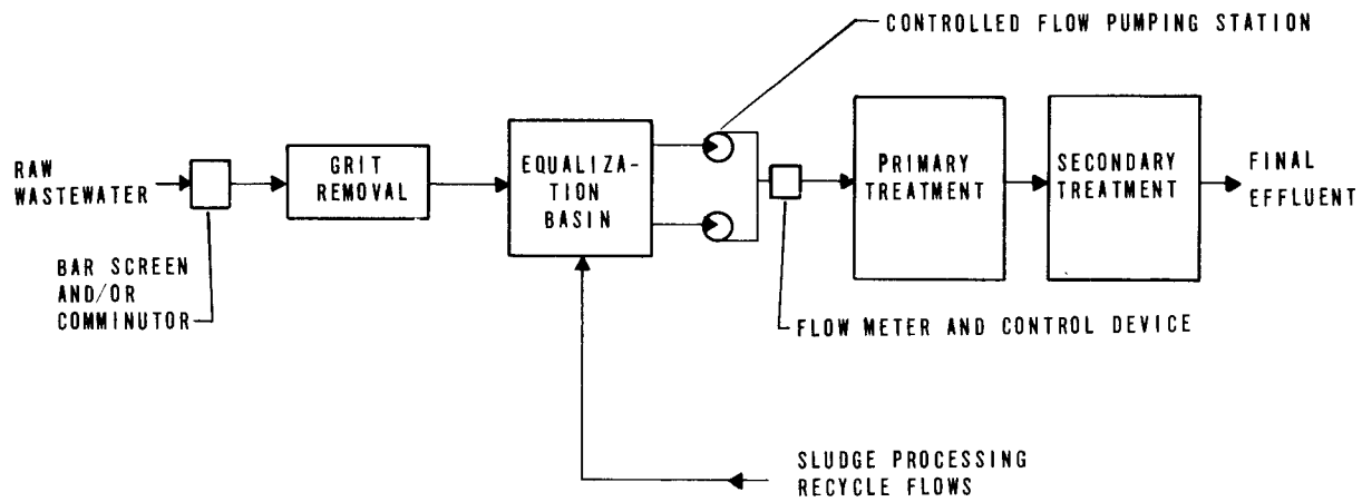
3-1a IN-LINE EQUALIZATION
