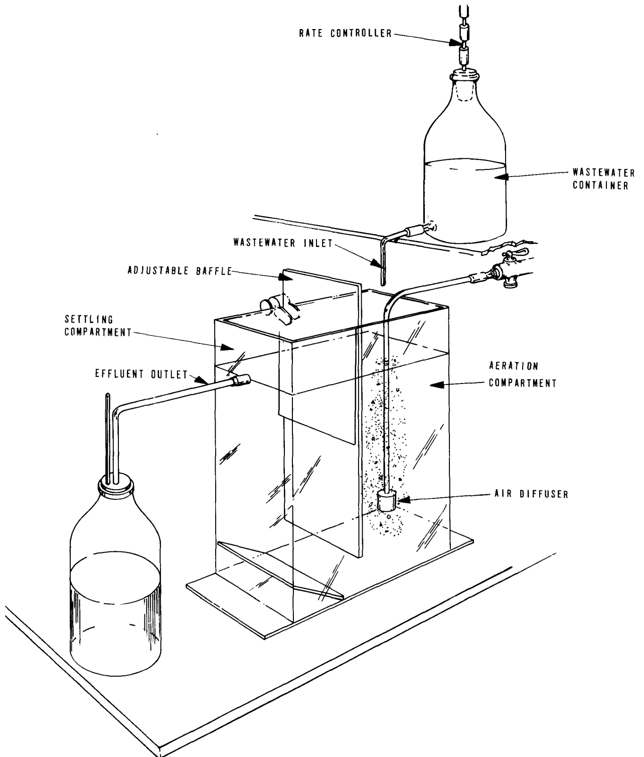
FIGURE 5-11 BENCH-SCALE AERATION UNIT
