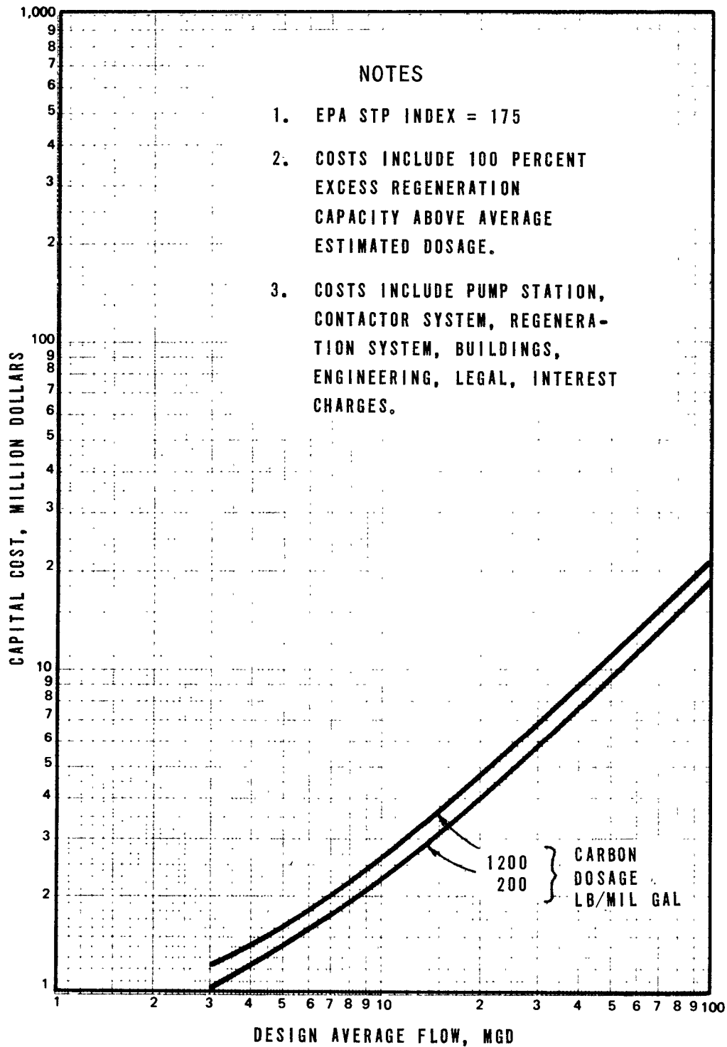
FIGURE 7-6 TOTAL CAPITAL COSTS FOR CARBON TREATMENT (2)
