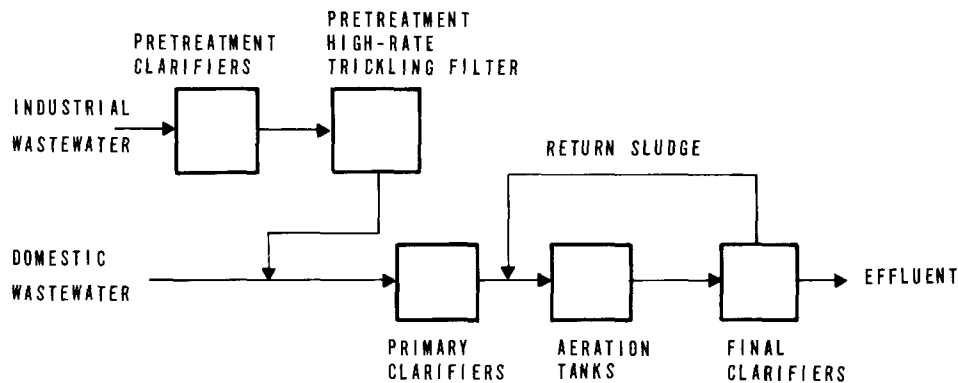
FIGURE 13-8 CASE HISTORY NO.8 FLOW DIAGRAM
