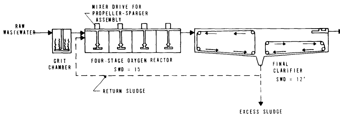
ELEVATION TREATMENT SYSTEM AFTER UPGRADING TO OXYGENATION (31)
