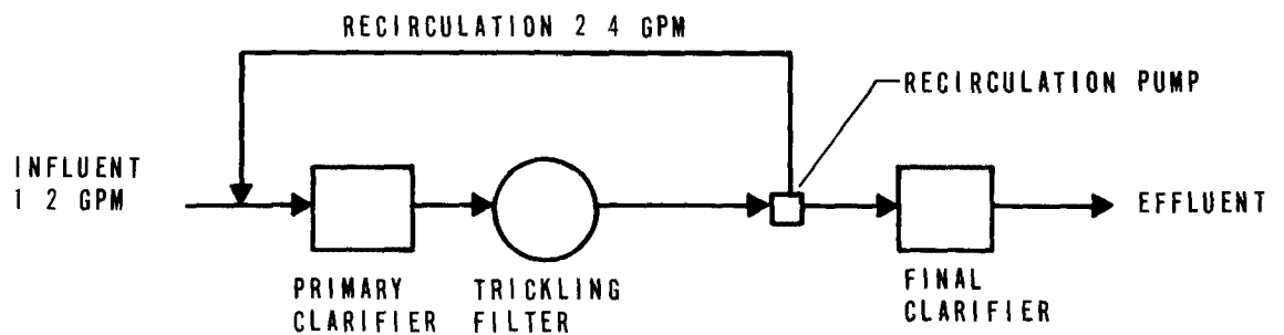
TREATMENT SYSTEM PERFORMING AS SINGLE-STAGE TRICKLING FILTER SYSTEM (ONE OF TWO DUPLICATE TRAINS)
