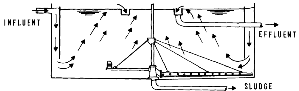
6-1b CIRCULAR RIM-FEED, CENTER TAKE-OFF CLARIFIER WITH A HYDRAULIC SUCTION SLUDGE REMOVAL SYSTEM
