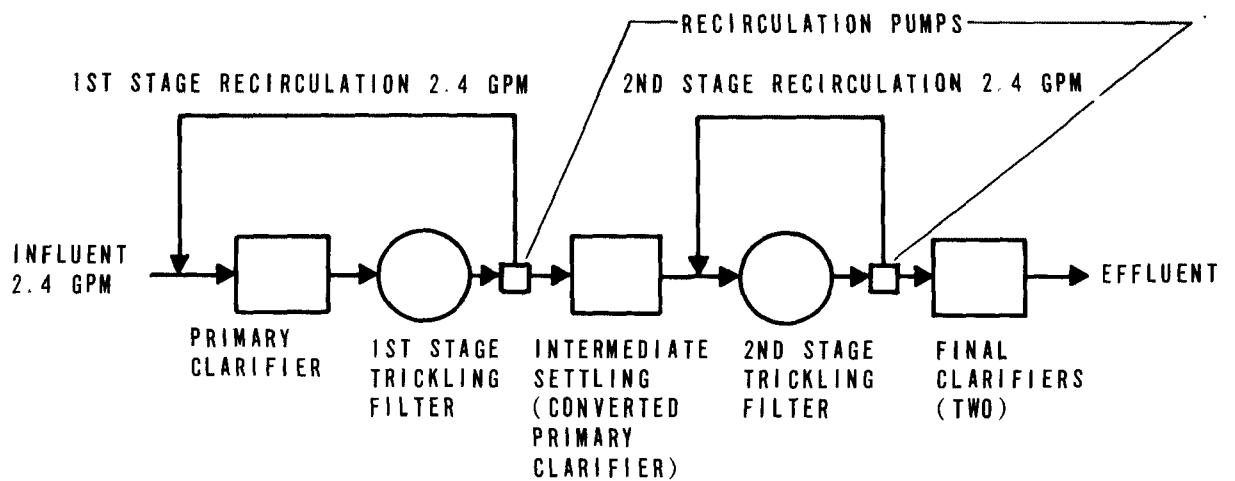
TREATMENT SYSTEM MODIFIED TO TWO-STAGE TRICKLING FILTER SYSTEM
