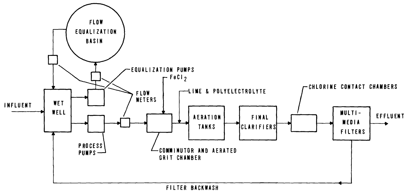
FIGURE 3-7 WALLED LAKE-NOVI WASTEWATER TREATMENT PLANT
