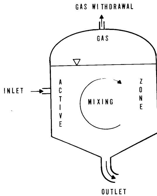
HIGH-RATE DIGESTER
