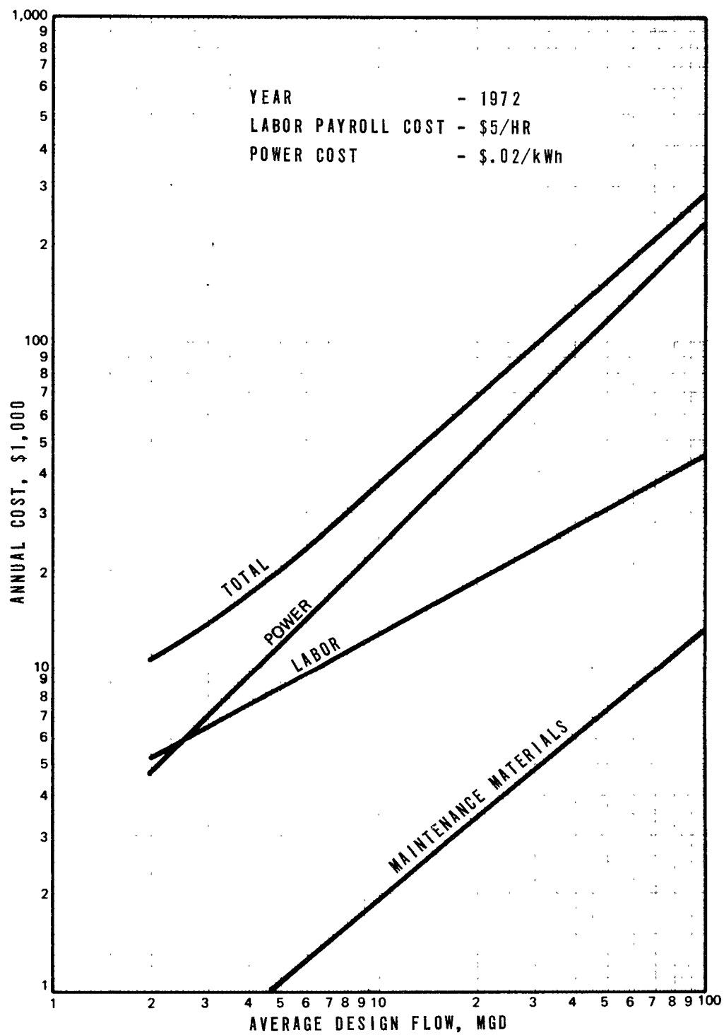
FIGURE 7-7 CARBON ADSORPTION OPERATION AND MAINTENANCE COSTS (2)
