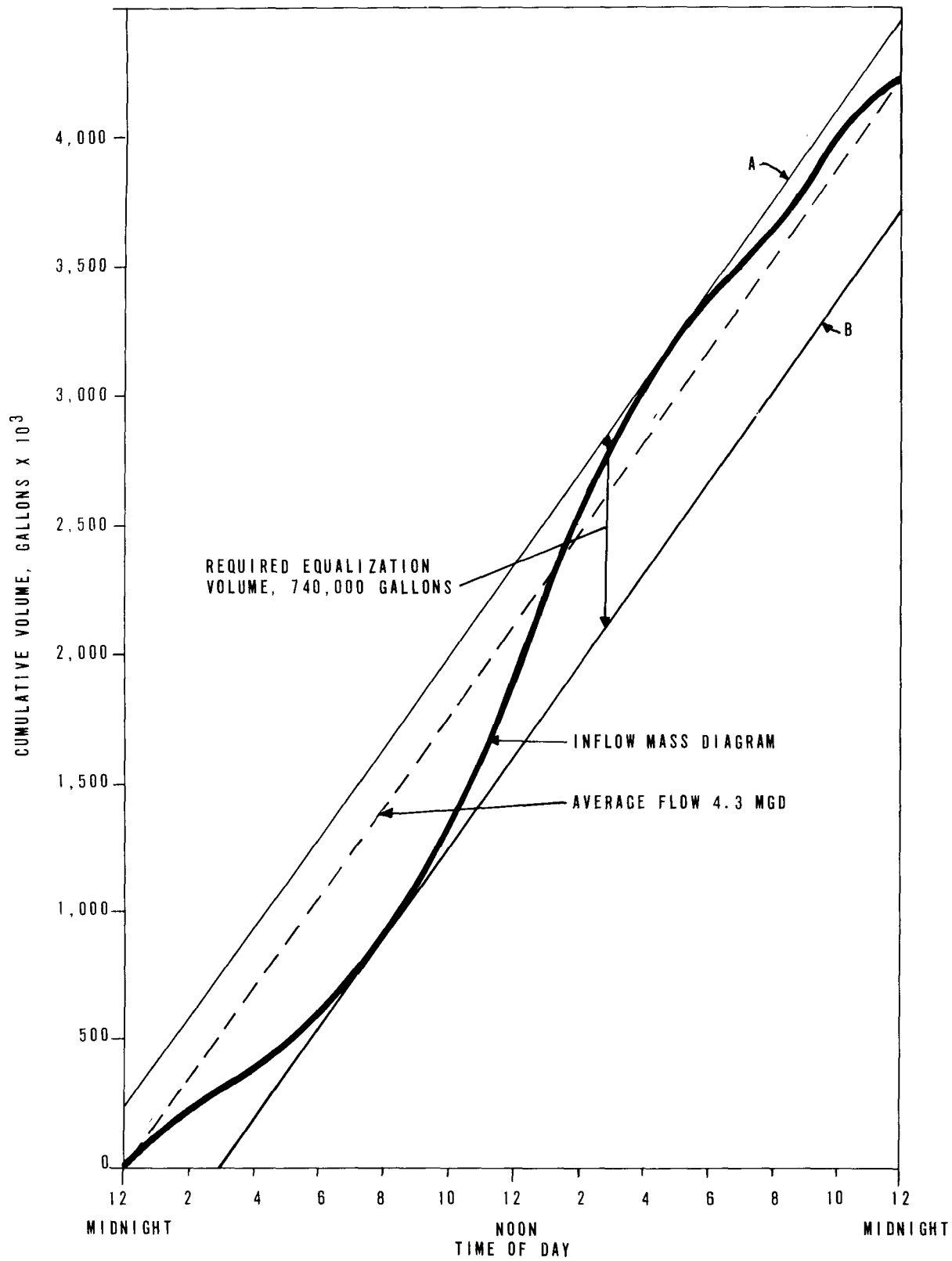
FIGURE 3-3 HYDROGRAPH FOR TYPICAL DIURNAL FLOW
