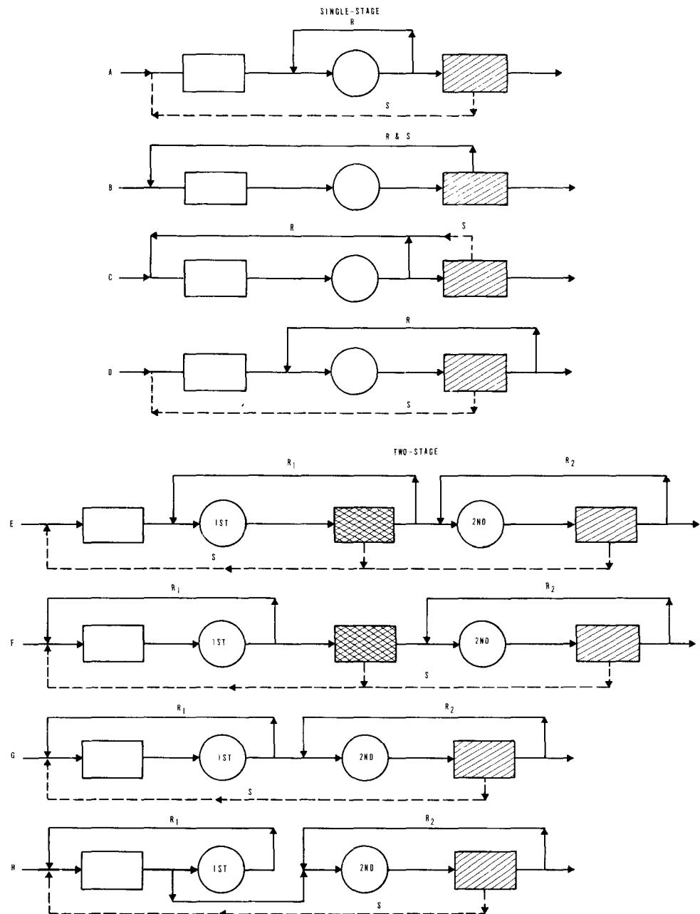
FIGURE 4-2 COMMON FLOW DIAGRAMS FOR SINGLE AND TWO-STAGE HIGH-RATE TRICKLING FILTERS (2)
