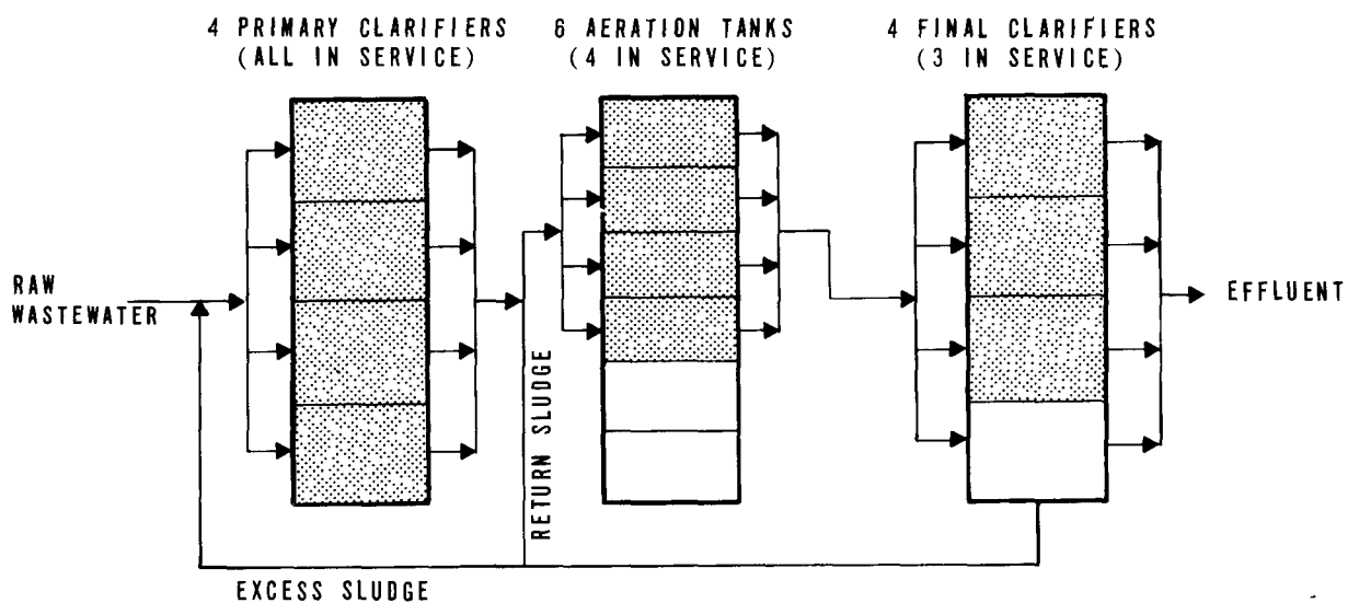
FLOW DIAGRAM AFTER PLANT MODIFICATION
