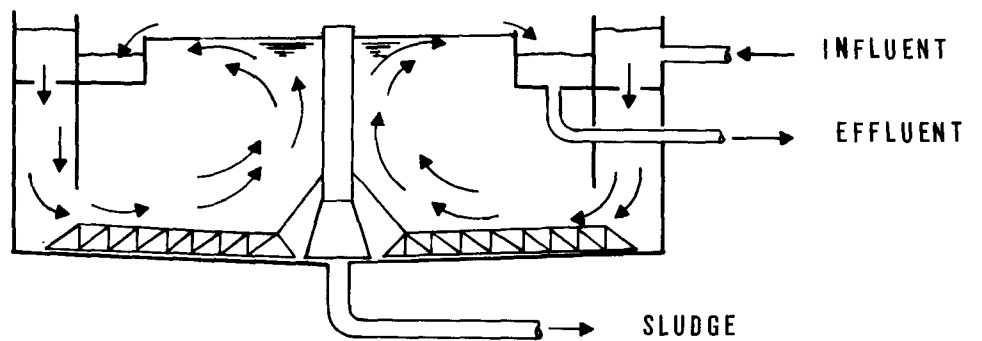
6-1c CIRCULAR RIM-FEED, RIM TAKE-OFF CLARIFIER
