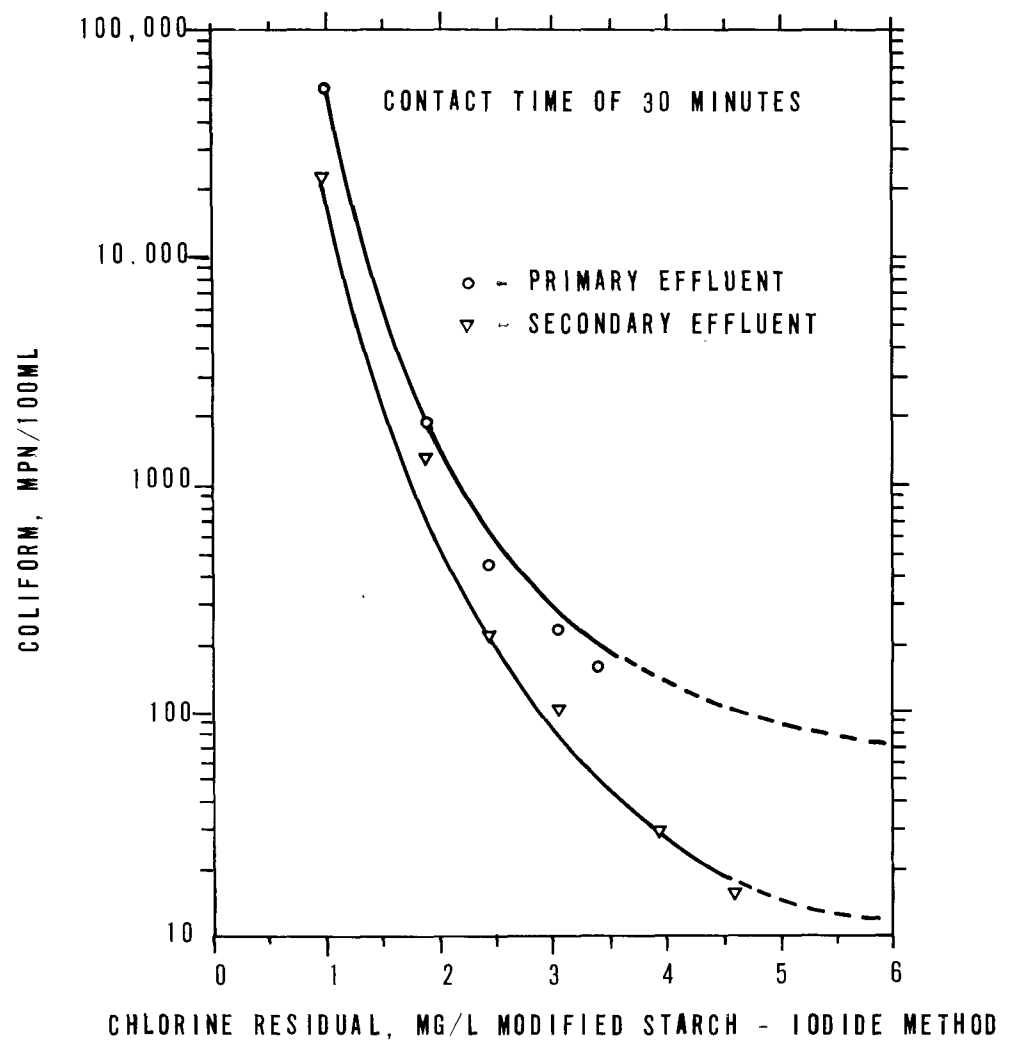
FIGURE 9-2 MPN COLIFORM VS. CHLORINE RESIDUAL (3)
