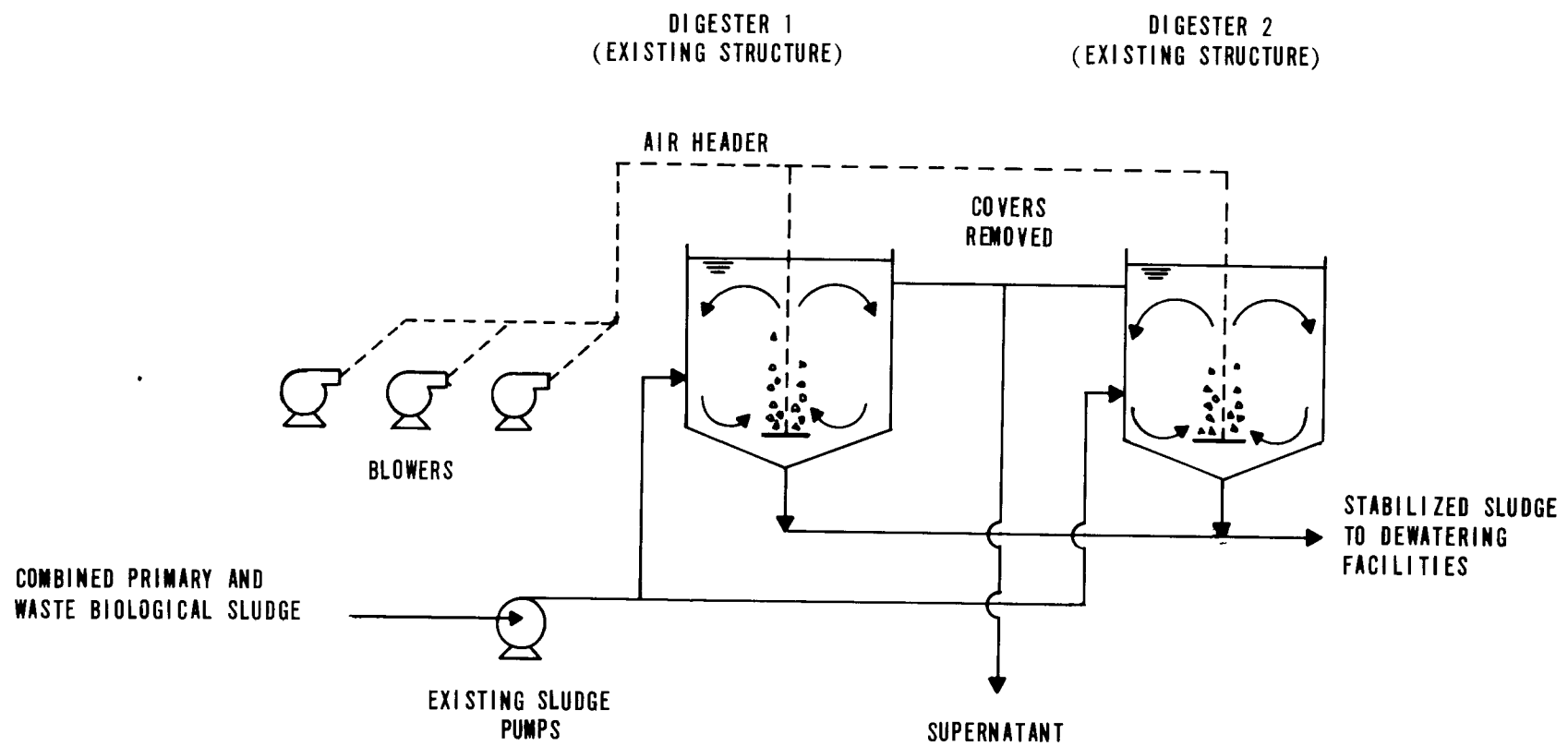
FIGURE 11-5 CONVERSION OF ANAEROBIC TO AEROBIC DIGESTION
