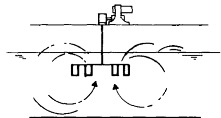
B-1 TURBINE TYPE AERATOR
