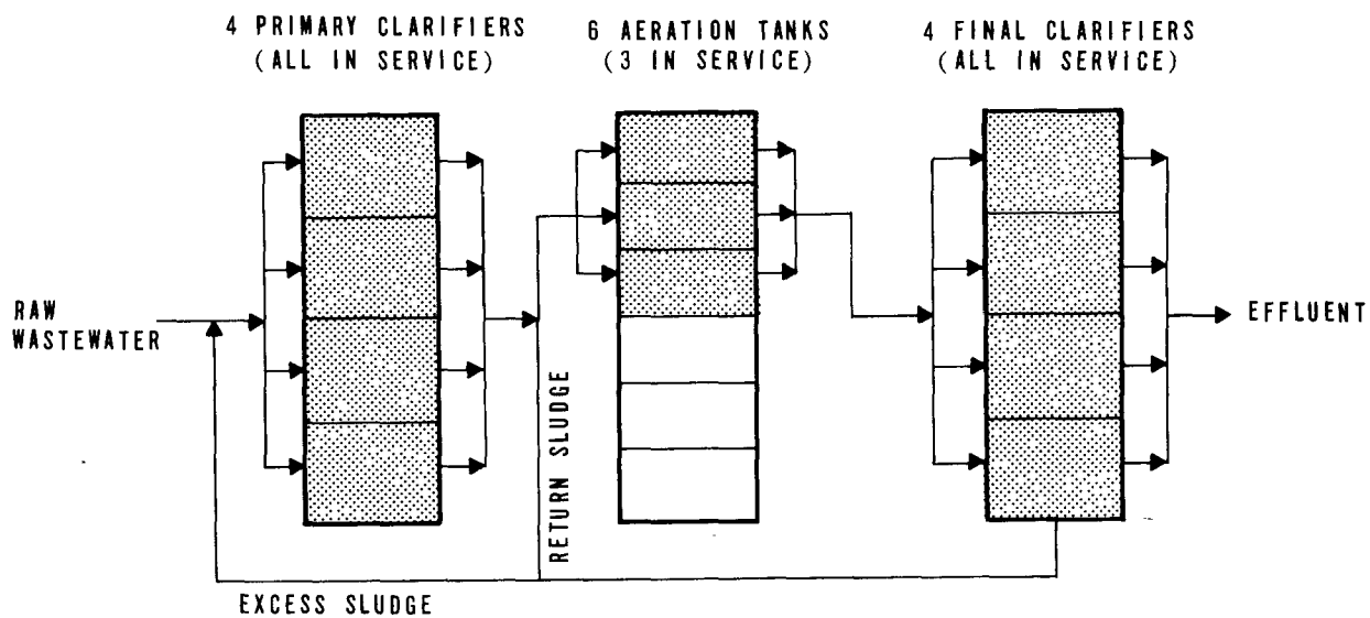
FLOW DIAGRAM BEFORE OPERATING MODIFICATION
