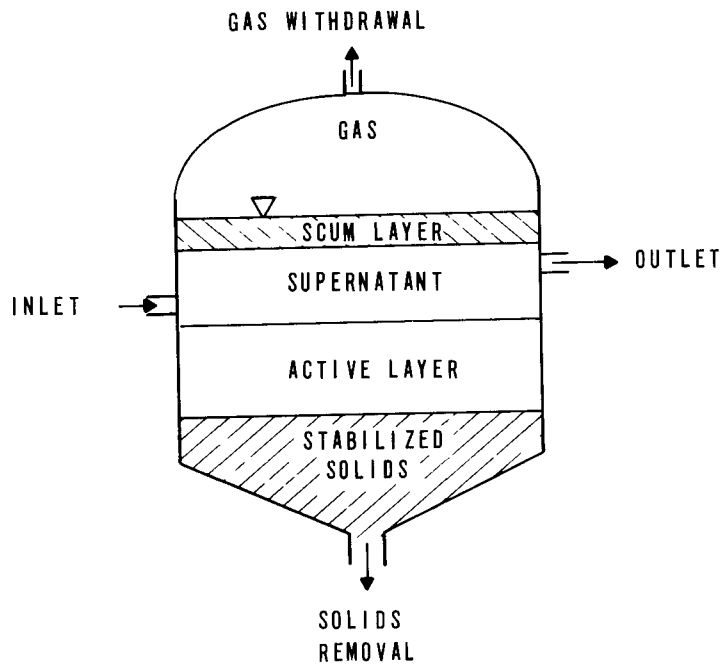
LOW-RATE DIGESTER
