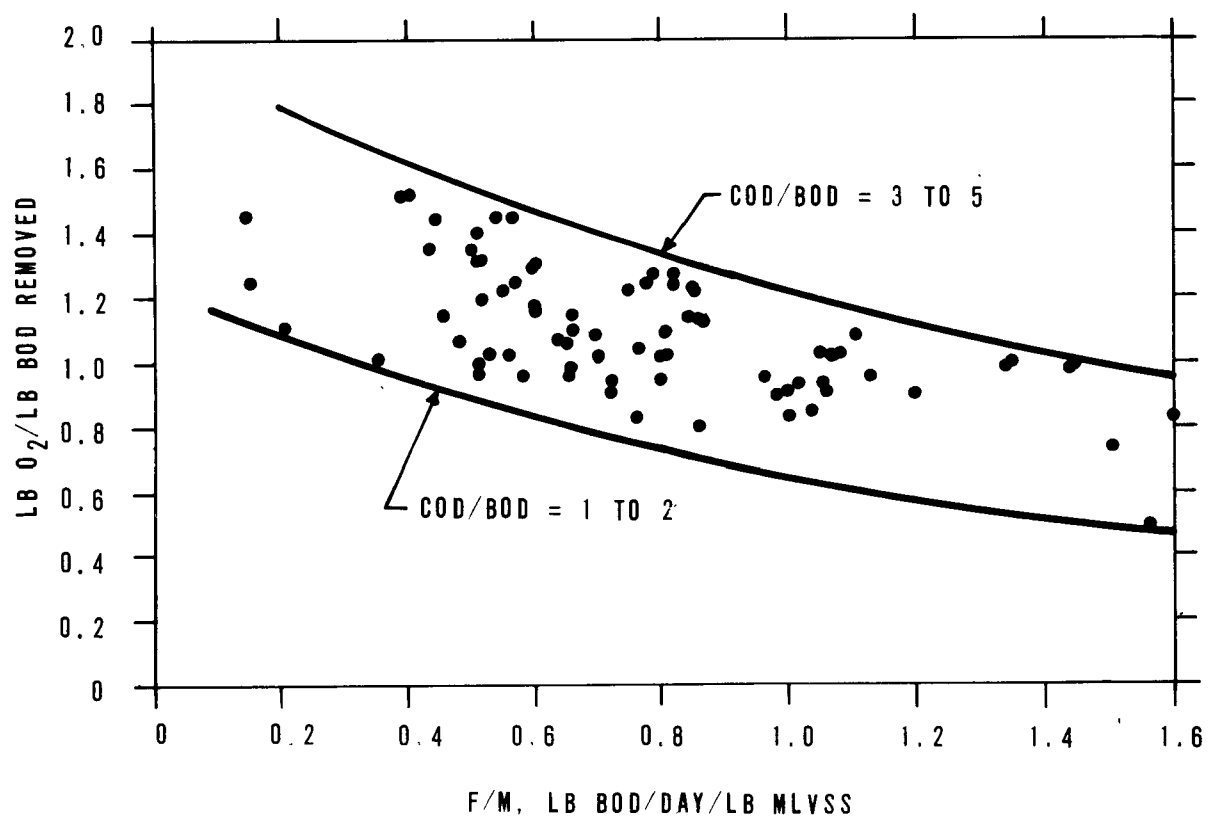
FIGURE 5-8 OXYGEN CONSUMPTION FOR PURE OXYGEN SYSTEMS RELATED TO ORGANIC LOADING (F/M) (33)
