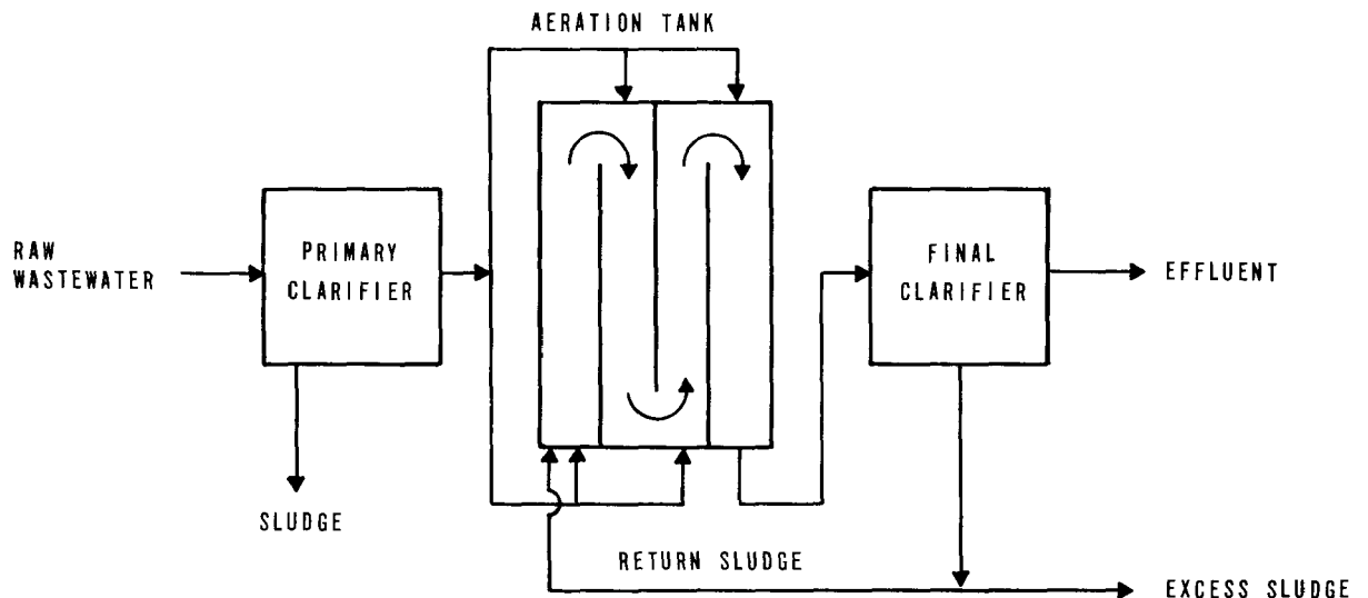
FIGURE 5-2 STEP AERATION PLANT
