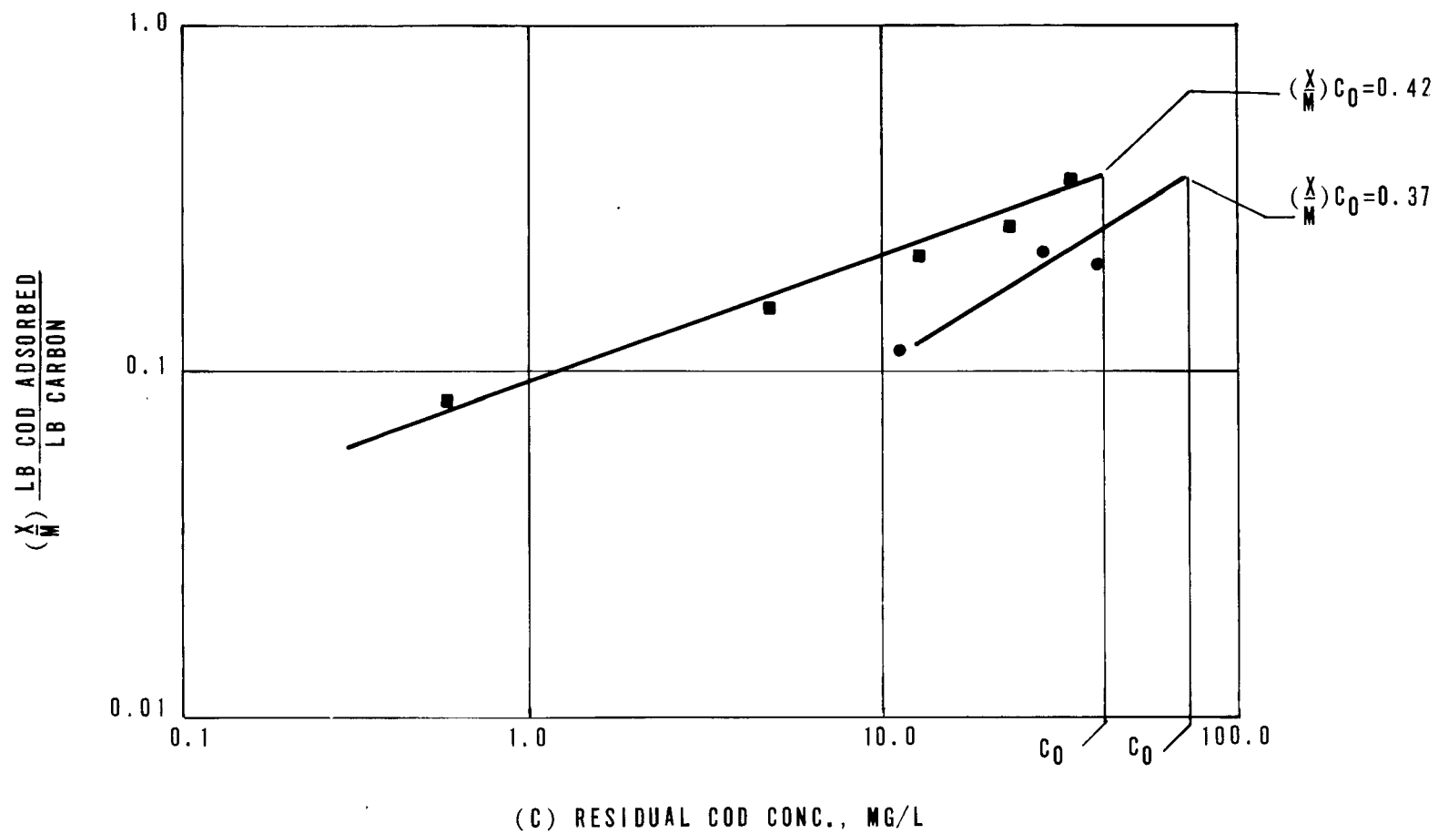
FIGURE 7-5 C O D ISOTHERMS USING VIRGIN CARBON AND DIFFERENT SECONDARY WASTEWATER EFFLUENTS (37)
