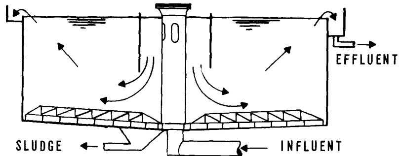
6-1a CIRCULAR CENTER-FEED CLARIFIER WITH A SCRAPER SLUDGE REMOVAL SYSTEM
