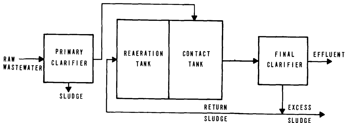
FIGURE 5-4 CONTACT STABILIZATION PLANT
