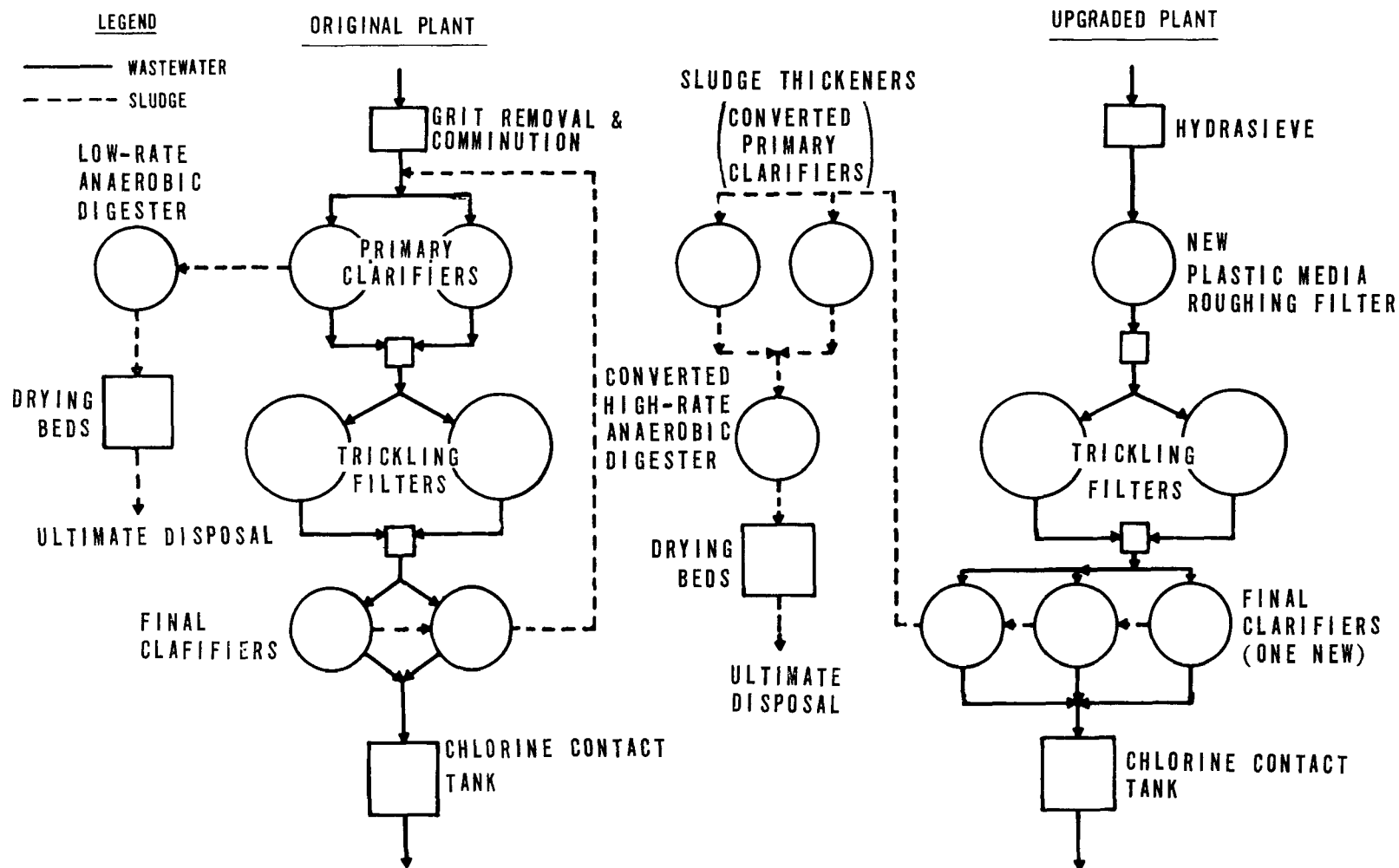
FIGURE 13-1 CASE HISTORY NO.1 COMPARISON OF ORIGINAL AND UPGRADED FLOW DIAGRAMS
