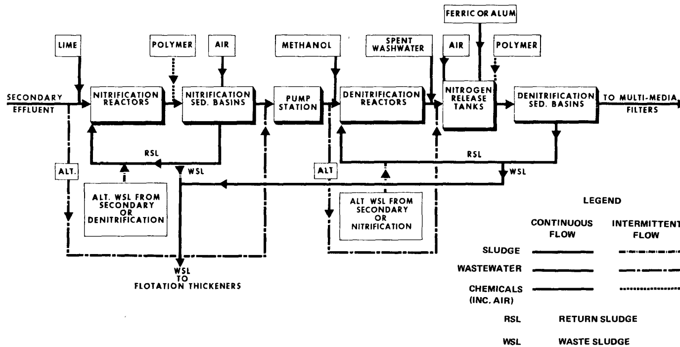
FIGURE 13-10 UPGRADING A MODIFIED AERATION SYSTEM FOR NUTRIENT REMOVAL FLOW DIAGRAM NITRIFICATION AND DENITRIFICATION SYSTEMS (10)
