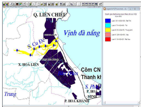
Figure 8. Partition diagram water quality indices WQI dry season.
