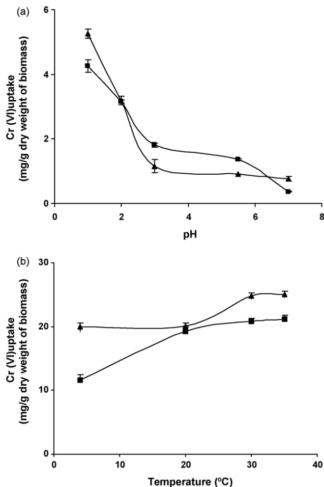
Fig. 1. (a) Effect of initial pH on Cr (VI) biosorption [ C_0 = 50 \text{ mg l}^{-1} , m (biomass) = 9.3 \text{ g l}^{-1} , 130 rpm, t (time) = 2 h, for Y. lipolytica NCIM 3589 (▲) and NCIM 3590 (■)]. (b) Effect of temperature on chromium (VI) biosorption [ C_0 = 200 \text{ mg l}^{-1} , m = 7.42 \text{ g l}^{-1} , 130 rpm, t = 2 \text{ h} and T = 4, 20, 30 and 35^\circ\text{C} for Y. lipolytica NCIM 3589 (▲) and NCIM 3590 (■)].
