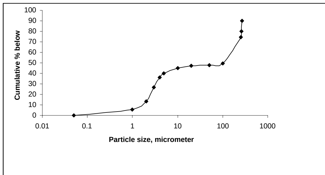
Figure 3: Particle Size Distribution of Sludge
