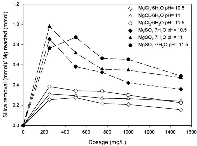
Fig. 4 mmol of silica removed per mmol of magnesium reacted at different initial pHs with \text{MgCl}_2 \cdot 6\text{H}_2\text{O} or \text{MgSO}_4 \cdot 7\text{H}_2\text{O} .
