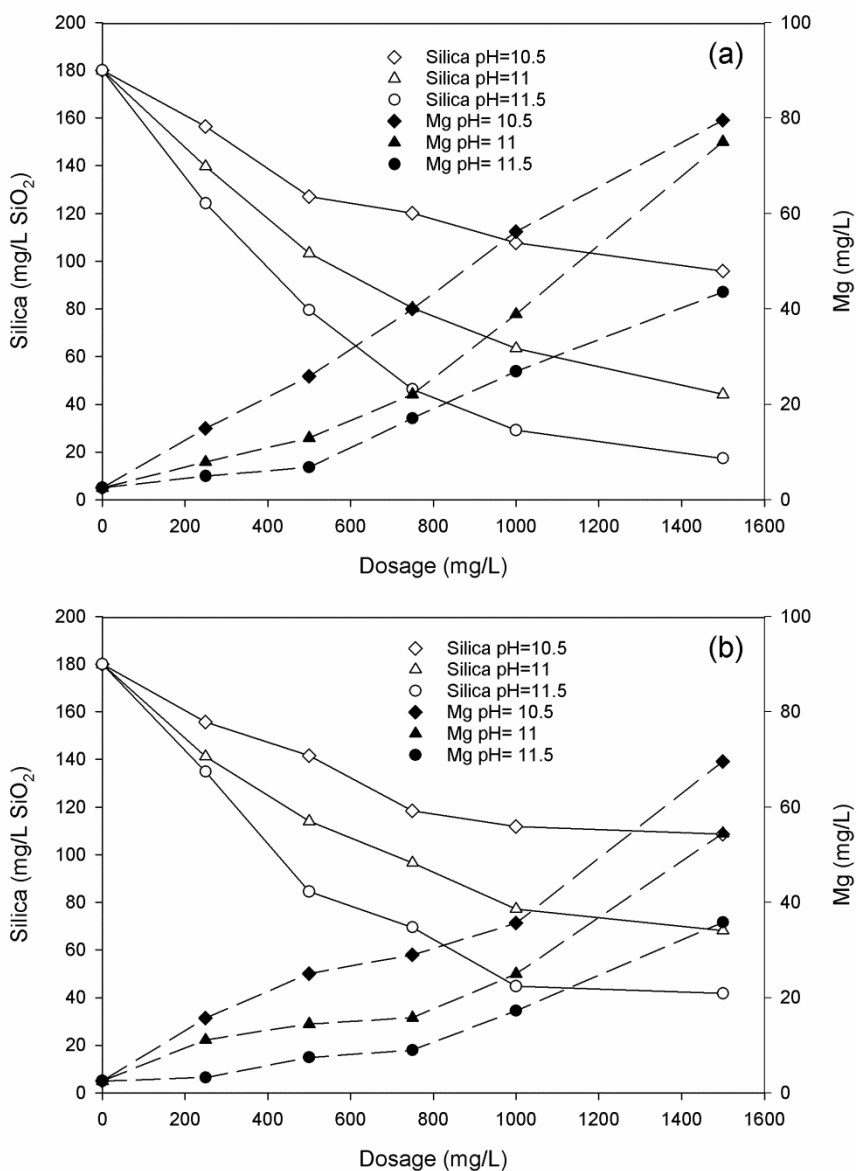
Fig. 2 Silica removal vs. dosage of (a) MgCl 2 ·6H 2 O and (b) MgSO 4 ·7H 2 O, at different initial pHs.
