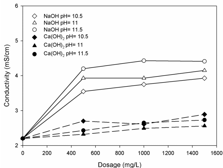
Fig. 6 Conductivity of treated waters vs. \text{MgCl}_2 \cdot 6\text{H}_2\text{O} dosage at different initial pHs with \text{Ca(OH)}_2 or NaOH as pH regulators.
