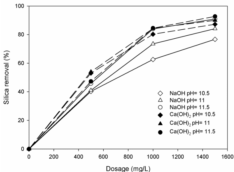
Fig. 5 Silica removal versus \text{MgCl}_2 \cdot 6\text{H}_2\text{O} dosage at different initial pHs with \text{Ca}(\text{OH})_2 or NaOH as pH regulators.
