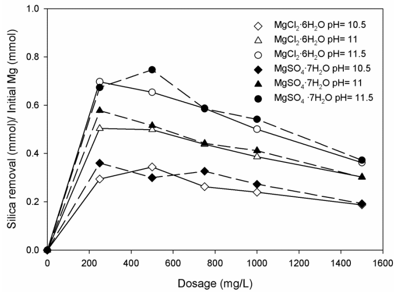
Fig. 3 mmol of silica removed per mg/L of initial magnesium at different initial pHs with \text{MgCl}_2 \cdot 6\text{H}_2\text{O} or \text{MgSO}_4 \cdot 7\text{H}_2\text{O} .
