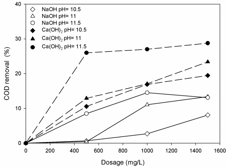
Fig. 7 COD removal vs. \text{MgCl}_2 \cdot 6\text{H}_2\text{O} dosage at different initial pHs with \text{Ca(OH)}_2 or NaOH as pH regulators.
