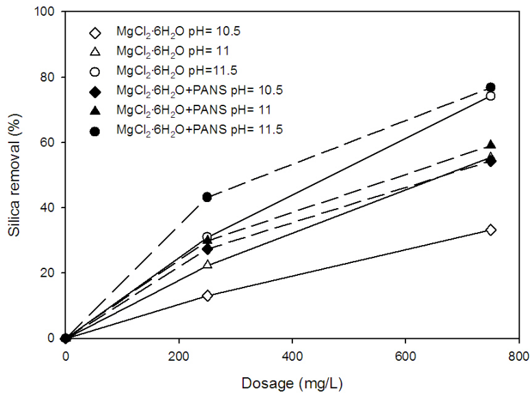
Fig. 8 Silica removal vs. \text{MgCl}_2 \cdot 6\text{H}_2\text{O} dosage at three pH with and without further coagulation treatment.
