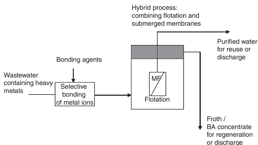
Figure 11 The integrated processes combining metal bonding and separation by a new hybrid process (for highly contaminated wastewater) (Mavrov et al., 2003).
