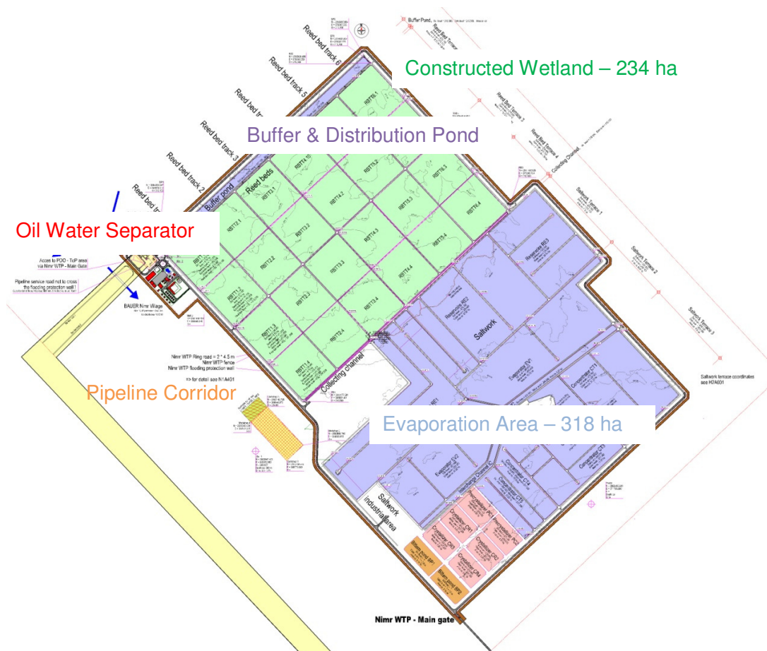
Figure 1: Nimr Water Treatment Plant Design
