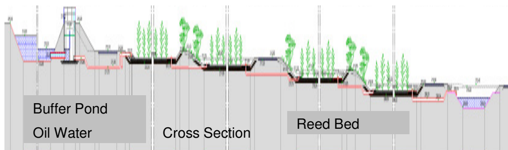
Figure 2: Nimr Water Treatment Plant – Wetland Cross Section
