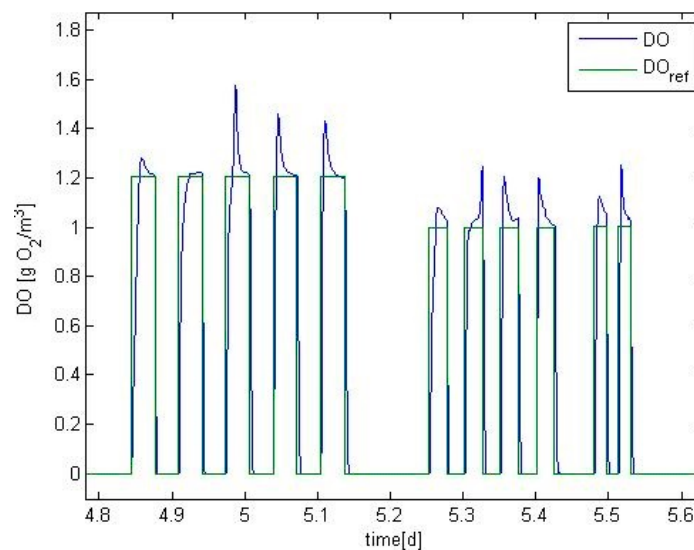
Figure 8. Dissolved oxygen—zoom.
