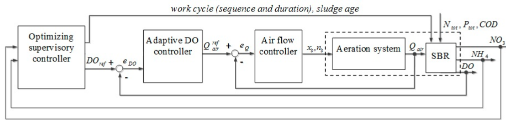
Figure 3. Structure of the hierarchical control system: Q_{air} , n_b , x_b , e_{DO} , e_Q , N_{tot} , P_{tot} , COD , NO_3 , NH_4 are the air flow [m 3 /h], blower speed [rpm], state of blower: on/off [-], error of DO [g O 2 /m 3 ], error of air flow [m 3 /h], total nitrogen [g N/m 3 ], total phosphorus [g P/m 3 ], chemical oxygen demand [g O 2 /m 3 ], nitrate concentration [g N/m 3 ], ammonia concentration [g N/m 3 ], respectively. The abbreviation for reference trajectory is designated as ref .
