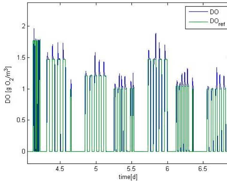
Figure 7. Dissolved oxygen.
