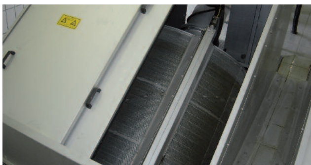
ROTAMAT® Rotary Drum Fine Screen Ro 2 installed in the channel with a movable stainless steel cover, size 600 to 3000
