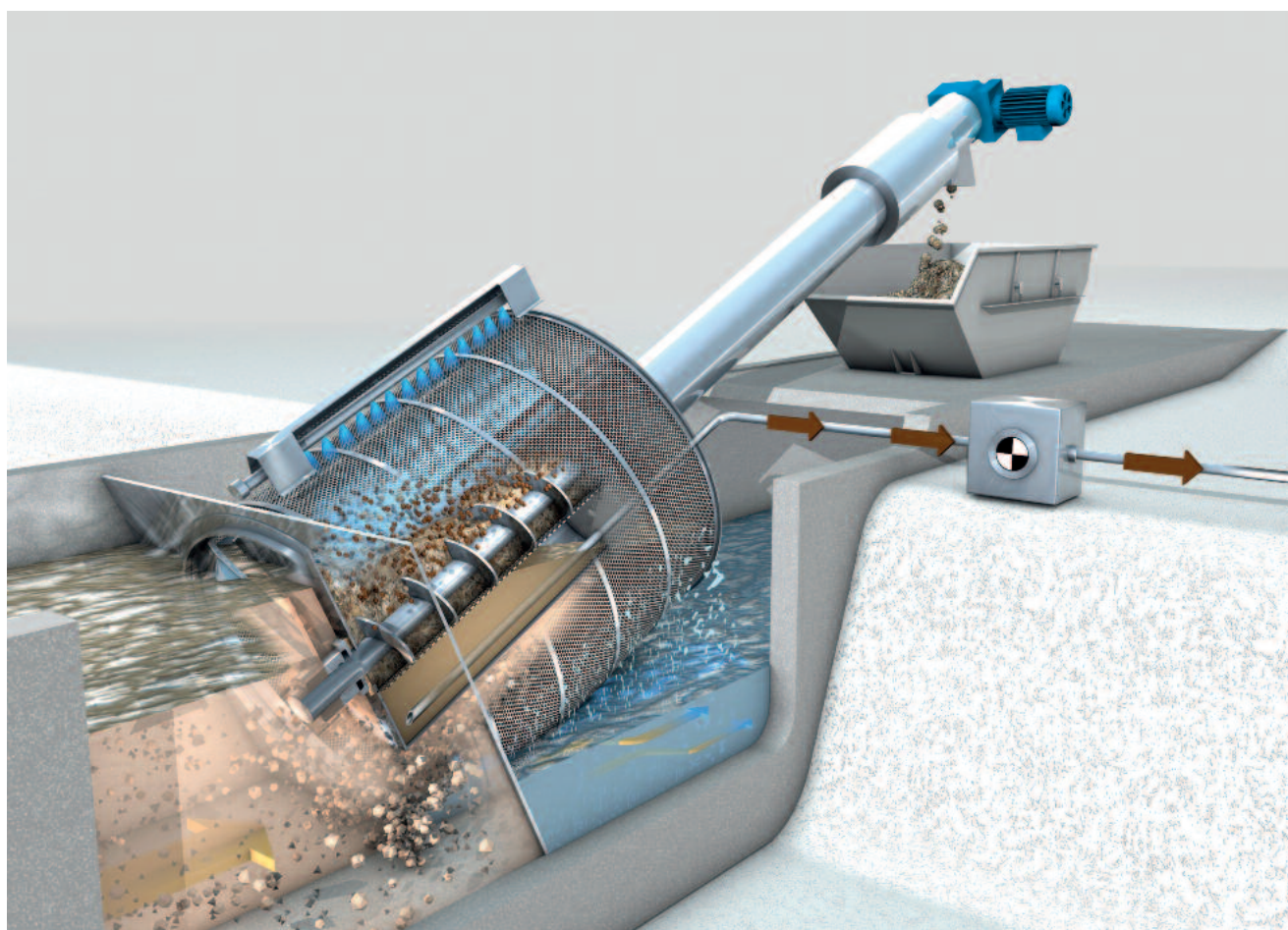
ROTAMAT® Rotary Drum Fine Screen Ro 2 / RPPS-PRO design
