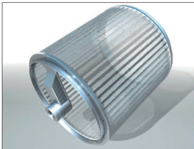
Schematic drawing of a ROTAMAT® Perforated Plate Screen RPPS-Star Screen with folded screen basket surface
