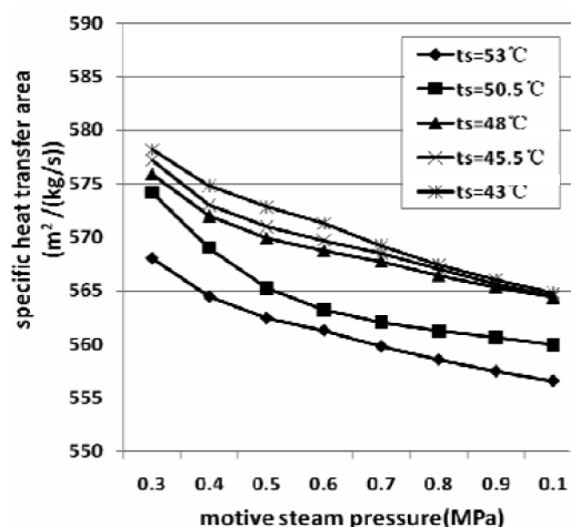
Fig. 7. Effects of motive steam pressure and suction steam temperature on specific heat transfer area.
