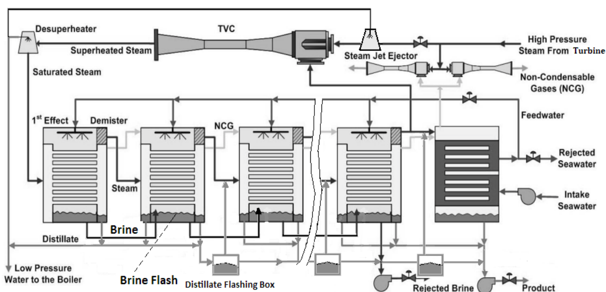
Fig. 1. Schematics of the MED-TVC system.
