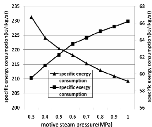
Fig. 5. Effects of motive steam pressure on specific exergy consumption and specific energy consumption.
