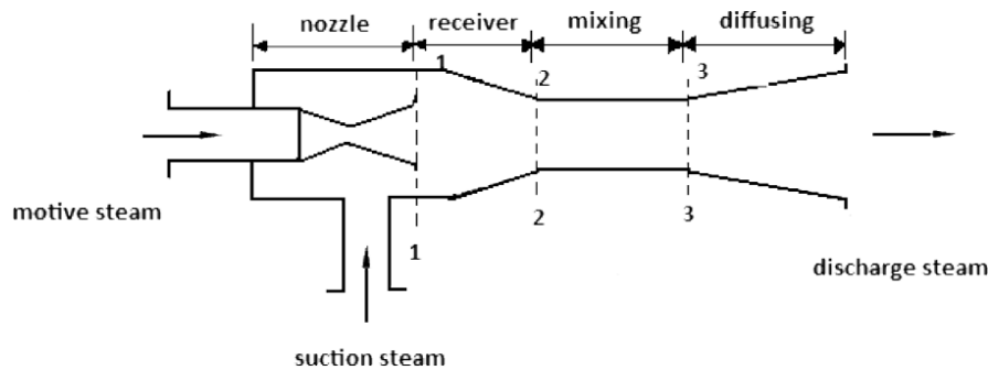
Fig. 2. Schematics of the thermal compressor.
