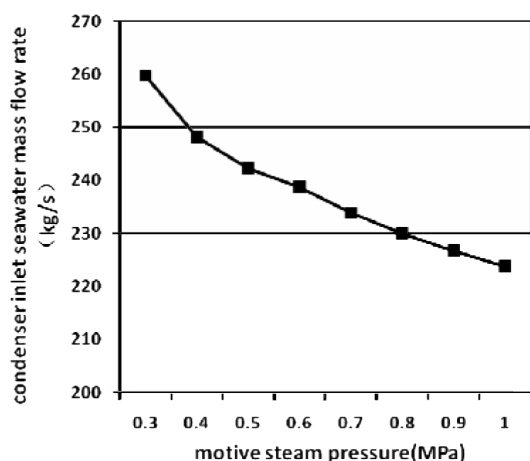
Fig. 6. Effects of motive steam pressure on condenser inlet seawater mass flow rate.
