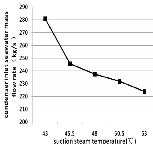
Fig. 11. Effect of suction steam temperature of the condenser inlet seawater mass flow rate.
