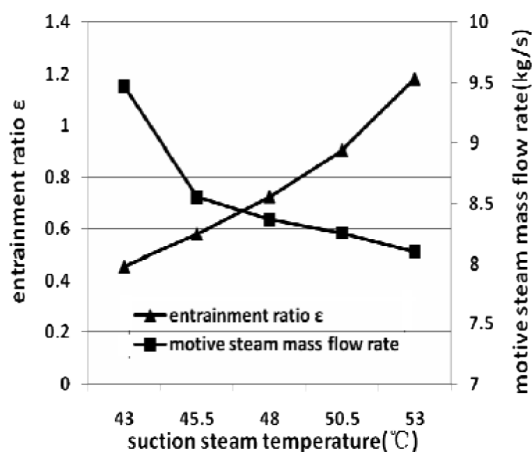
Fig. 8. Effects of suction steam temperature on motive steam mass flow rate and entrainment ratio \epsilon .
