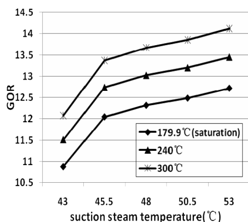
Fig. 10. Effects of suction steam temperature and degree of superheat of motive steam on the GOR.
