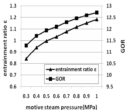
Fig. 4. Effect of motive steam pressure on entrainment ratio \varepsilon and the GOR.
