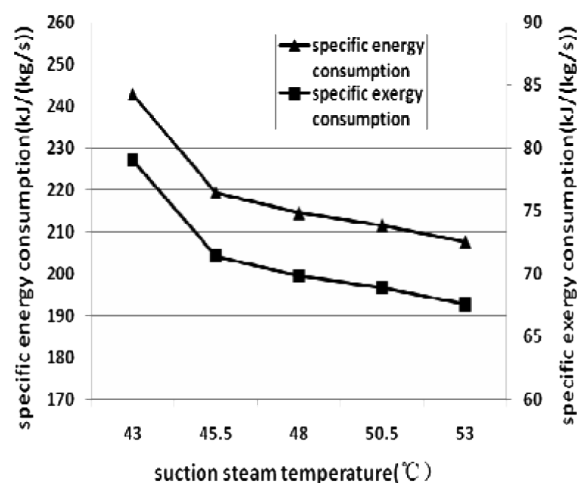
Fig. 9. Effects of suction steam temperature on specific exergy consumption and specific energy consumption.
