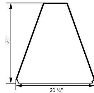
Lifting Handle
