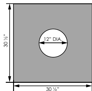
Base Plate
