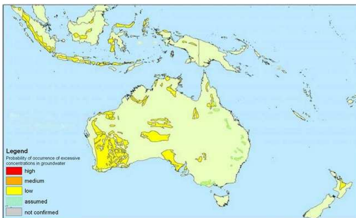
Figure 9 Fluoride in groundwater in Australia
