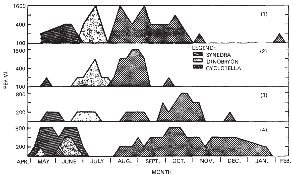
Figure 61.—Pulses, over a four year period, of three taste and odor algae in a water supply reservoir.
