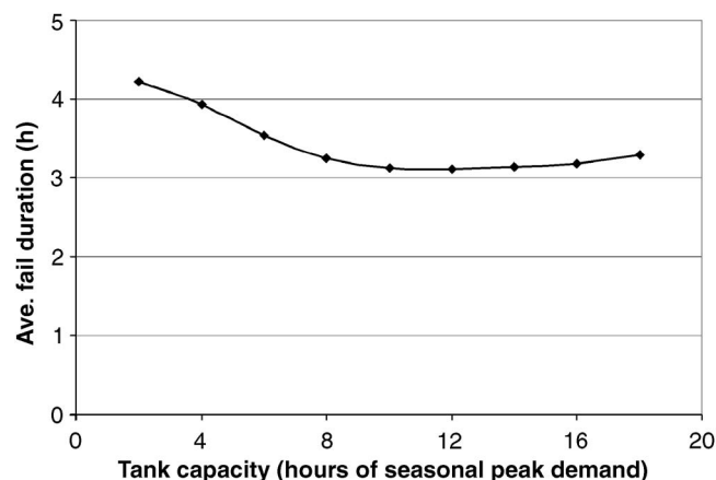
Fig. 3. Average tank failure duration as a function of the tank capacity
