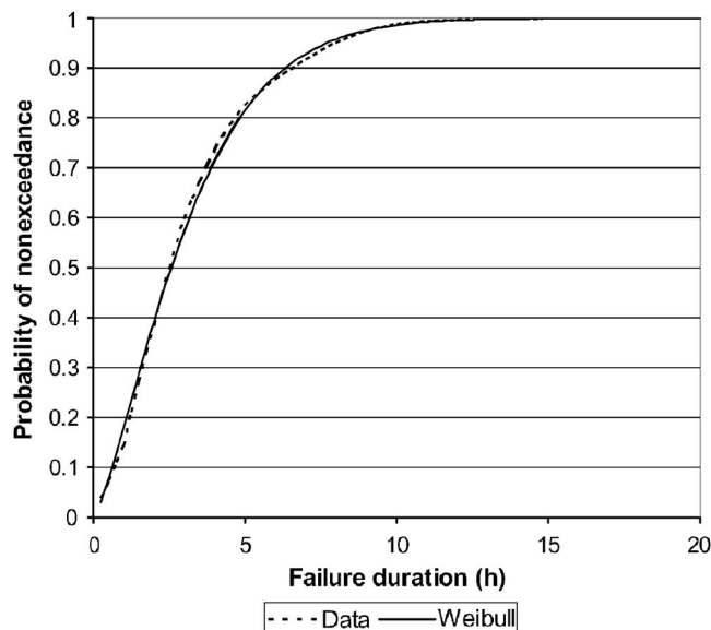
Fig. 4. Failure duration distribution for a tank with a capacity of 12 h of seasonal peak demand
