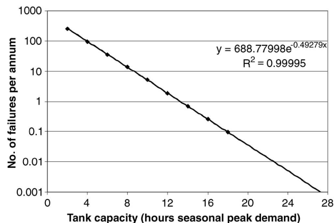
Fig. 2. Annual average number of tank failures as a function of the tank capacity
