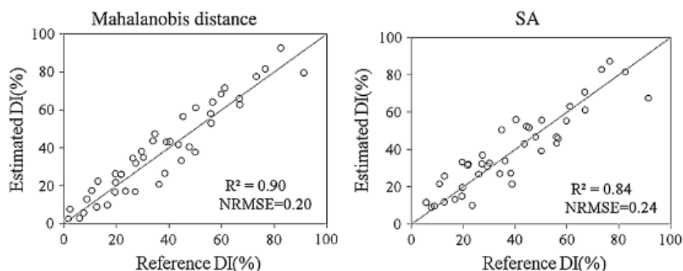
Fig. 11. Estimated DI(%) using simulated data
