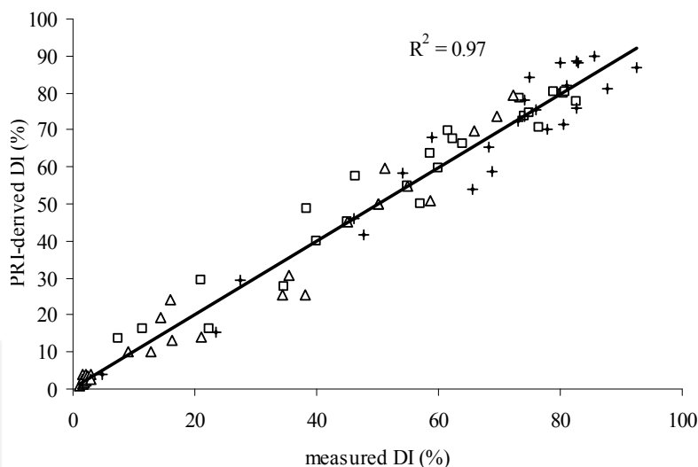
Fig. 5. Comparison of measured DI and PRI-estimated DI for 2003 Exp; \Delta = Jing 411; + = Xuezaao; \square = 98-100
