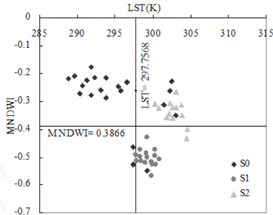
Fig. 23. Distribution of test sample plots in LST-MNDWI feature space
