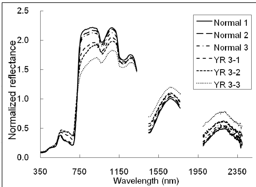
(b) Normalized spectra on 233 days after sowing
