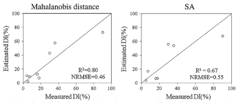
Fig. 12. Estimated DI(%) using field measurements
