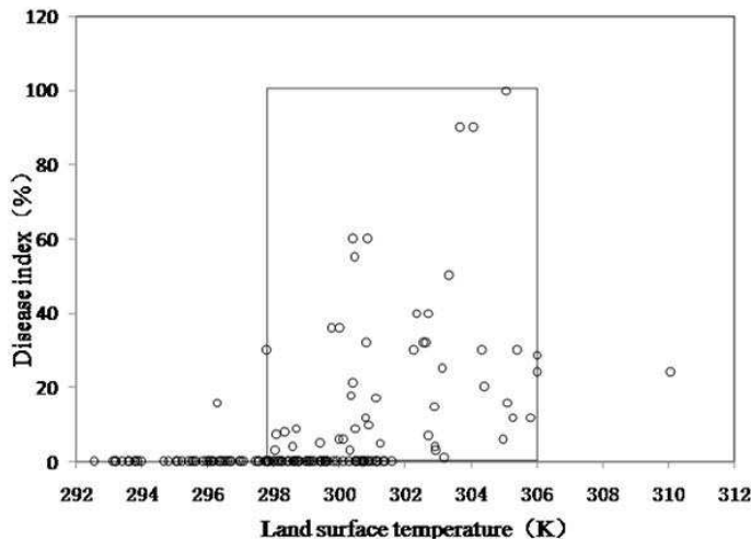
Fig. 13. The distribution of the investigation points
