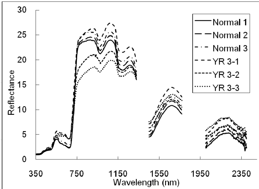
(a) Original spectra on 233 days after sowing
